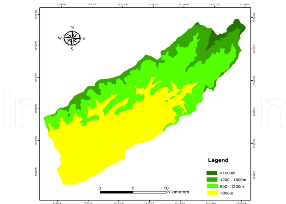
Figure 2. Elevation increases gradually towards northeast in the study area
