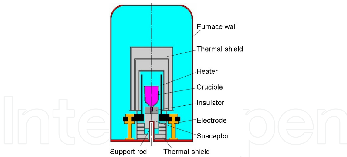
Figure 20. Schematic diagram of a TGT furnace.
