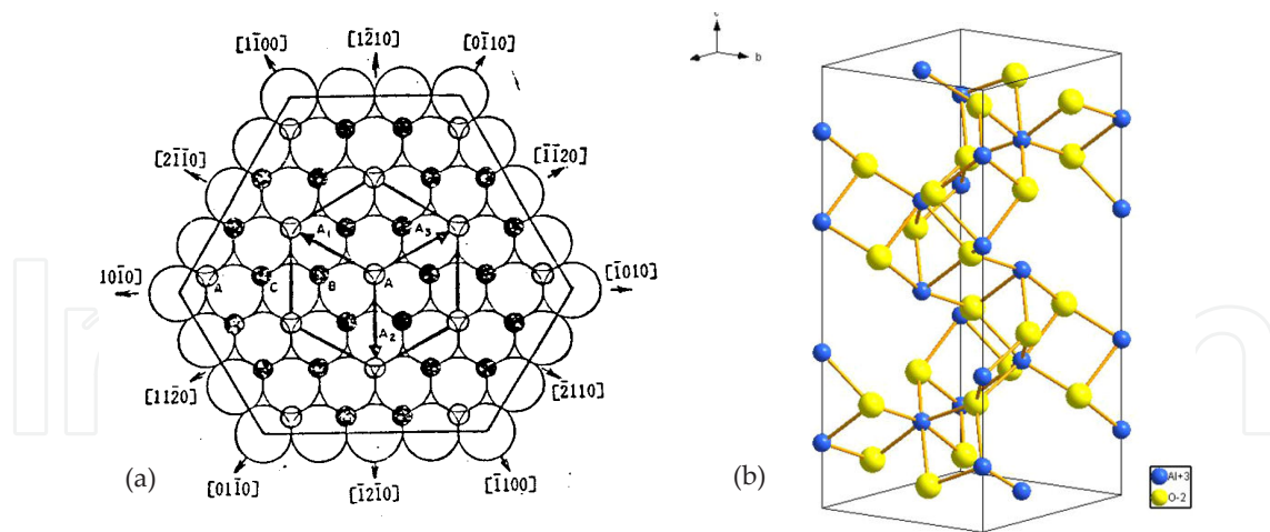
Figure 1. a) Schematic of the packing of O^{2-} ions in the sapphire cell, (b) Rhombodredal unite cell of the sapphire crystal.
