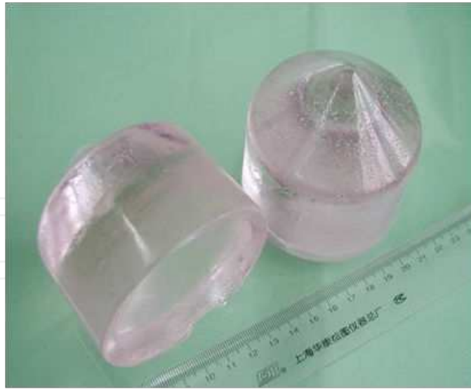
Figure 21. Sapphire crystals grown by TGT.
