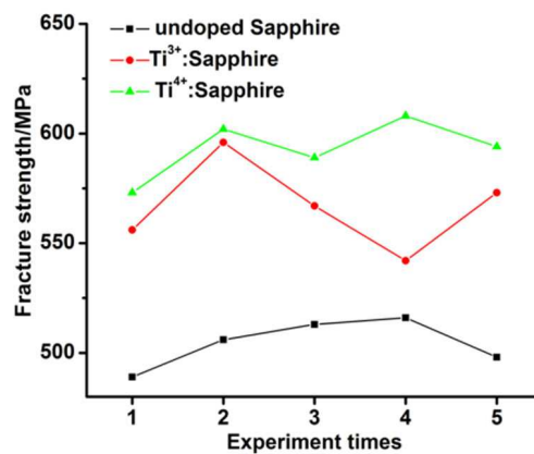
Figure 5. Fracture strength of Ti :sapphire and sapphire crystals.
