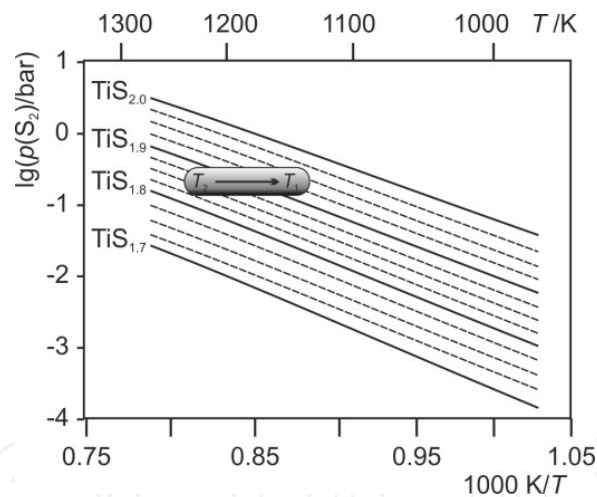
Figure 34. Phase barogram for the system Ti/S showing the co-existence pressures (according to 198) in the homogeneity range \text{TiS}_{2-\delta} . The phase relations in CVT experiments (950 to 850 °C) are visualized; graphic according to [16, 2].
