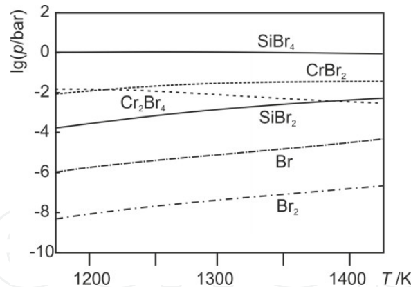
Figure 18. Composition of the gas phase for the transport of CrSi using bromine, according to [89].
