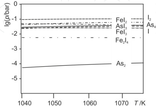
Figure 32. Composition of the gas phase for the transport of \text{FeAs}_2 using iodine, according to [2].
