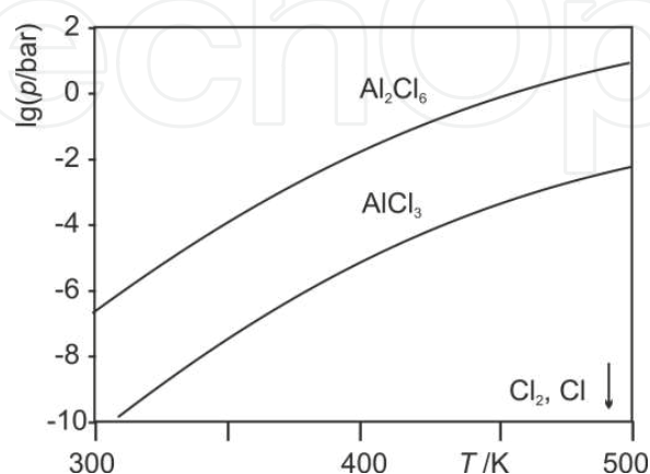
Figure 2. Composition of the gas phase of sublimation of \text{AlCl}_3 .
