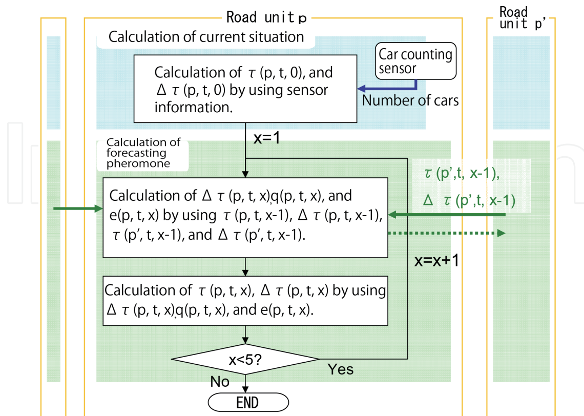
Figure 5. Flow chart for forecasting congestion
