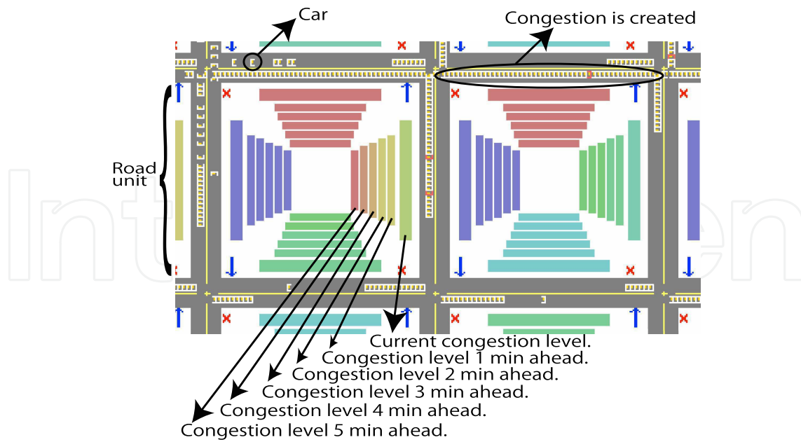
Figure 8. Forecasting scenario in simulator
