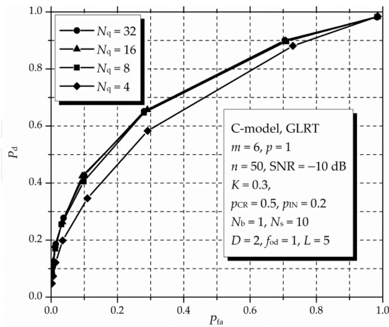
Figure 15. ROC curves for GLRT with IN under N_q variations for R -model.
