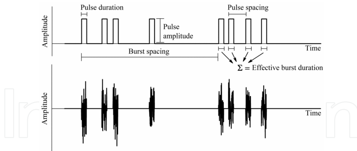
Figure 4. Gating waveform (top) and impulsive noise waveform (bottom) (From [26]).
