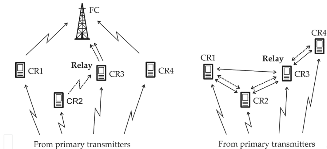
Figure 2. Classification of cooperative spectrum sensing (left) centralized, (right) distributed.
