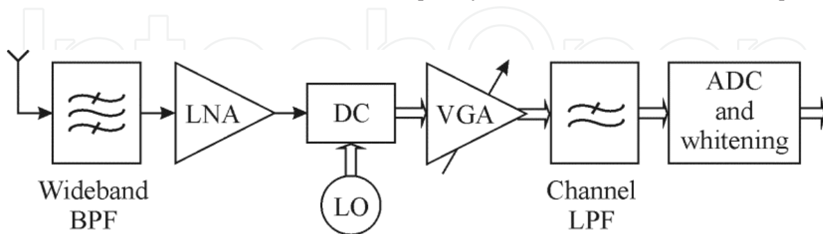
Figure 3. CR receiver diagram (adapted from [28]).
