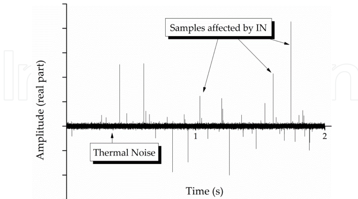
Figure 5. Illustration of the compound (thermal plus impulsive) noise waveform generated by the simulation platform.
