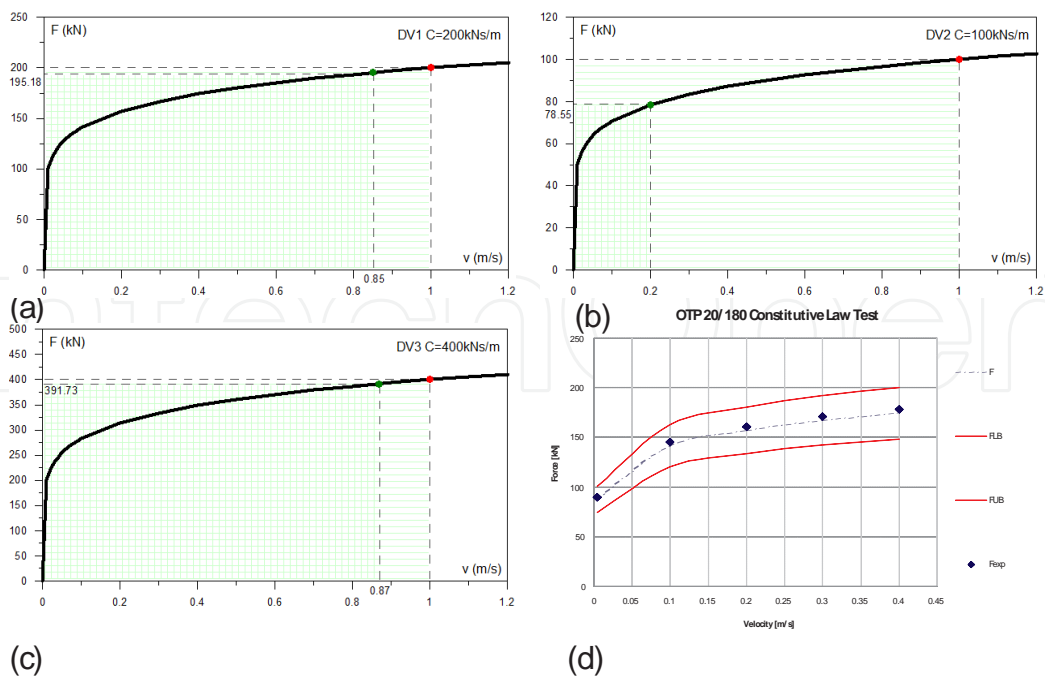
Figure 6. Design force-velocity relations for the three types of nonlinear viscous dampers; a) DV1 b) DV2 c) DV3 d) experimental data from the characterization tests [7].
