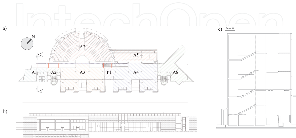
Figure 2. Edifice A: a) plan view at the main entrance level 0, b) facade view c) section A-A
