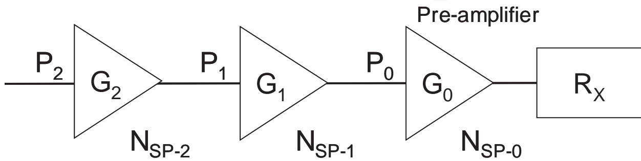
Figure 3. Cascading amplifiers.
