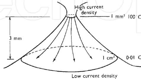
Figure 1. Principle of “current density” in diathermy electrocoagulation – heating effect in the stalk of the polyp (after Curtiss 1973)
