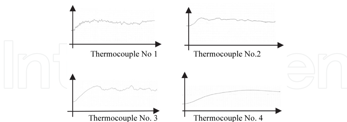
Fig. 8. Linear - Pulse Mode (10 pps) - Voltage changes ( \mu V) versus Time (sec.) for each thermocouple
