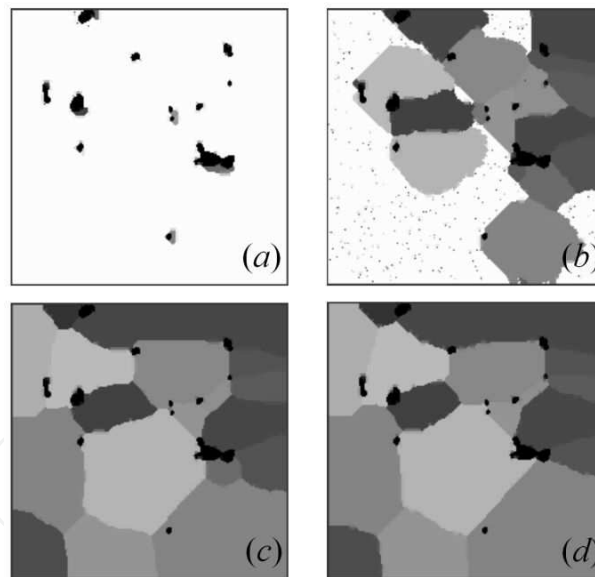
Figure 14. Simulated microstructural evolution with the presence of IMPs, (a) after 1500 TCs, (b) after 3000 TCs, (c) after 4000 TCs, (d) after 5000 TCs [39].
