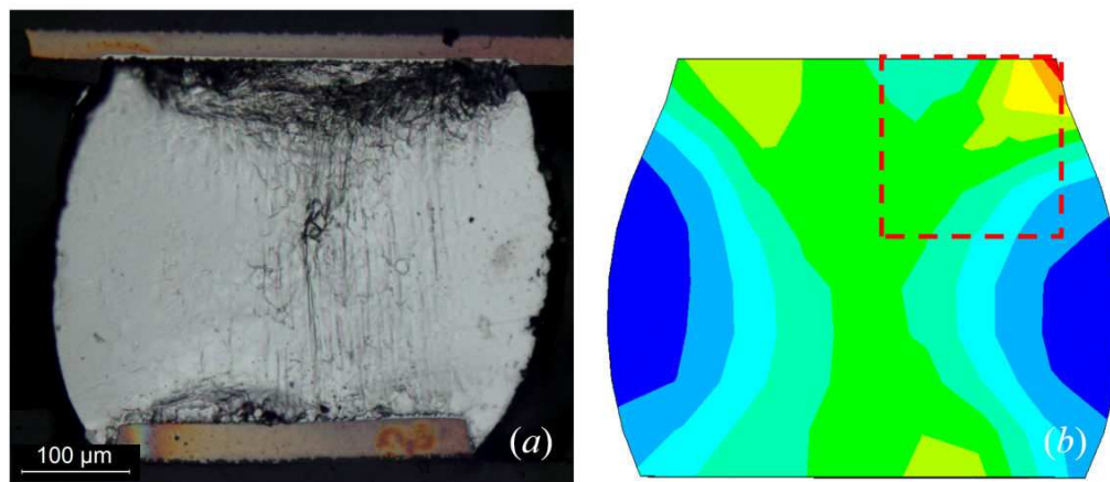
Figure 11. a) Plastic deformation of the solder interconnection after 1000 thermal cycles, (b) FEM-calculated inelastic strain energy density distribution, dashed rectangle shows the domain of the microstructural simulation [39].
