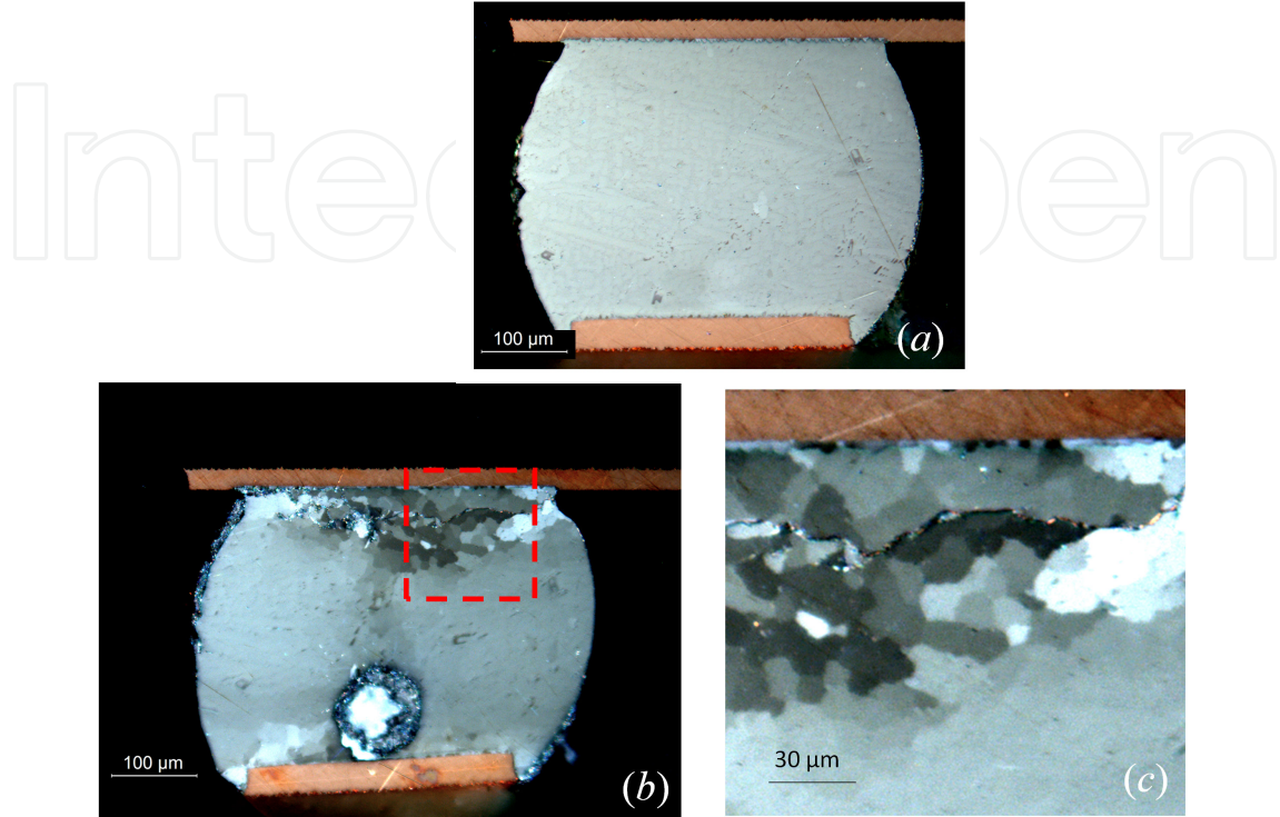
Figure 8. Microstructure of the outermost solder interconnection observed with polarized light (a) after solidification, (b) after 1000 thermal cycles observed with polarized light, (c) close-up view of the top right corner of the cross section [39].
