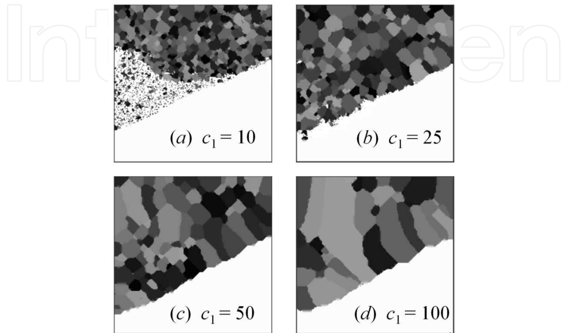
Figure 9. Simulated microstructures with four typical c_1 values [39].
