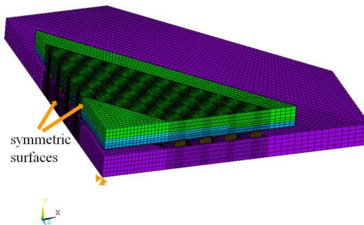
Figure 7. Finite element model for the thermomechanical calculation [39].
