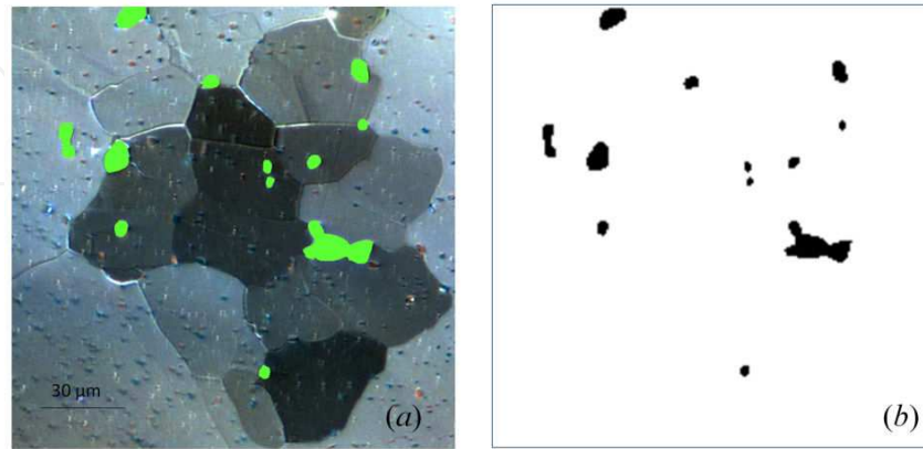
Figure 13. a) Micrograph shows IMP-affected recrystallization, (b) initial microstructure for the Monte Carlo simulation [39].
