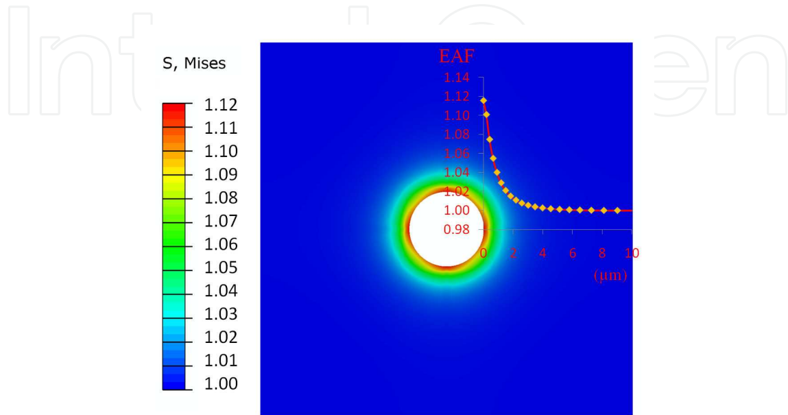
Figure 10. von Mises stress contour and 'EAF vs. distance' curve [39].
