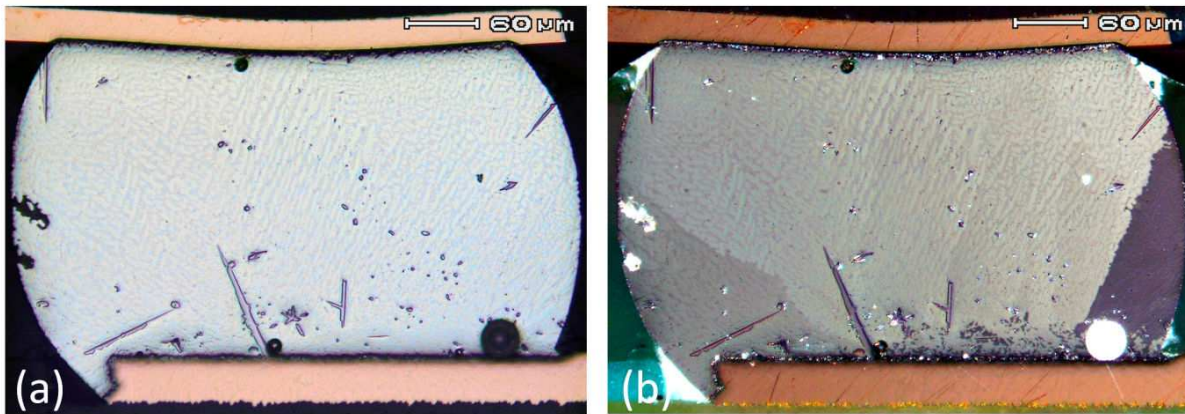
Figure 2. The as-solidified microstructure of a SnAgCu solder interconnection; (a) optical bright field image, (b) cross-polarized light image.
