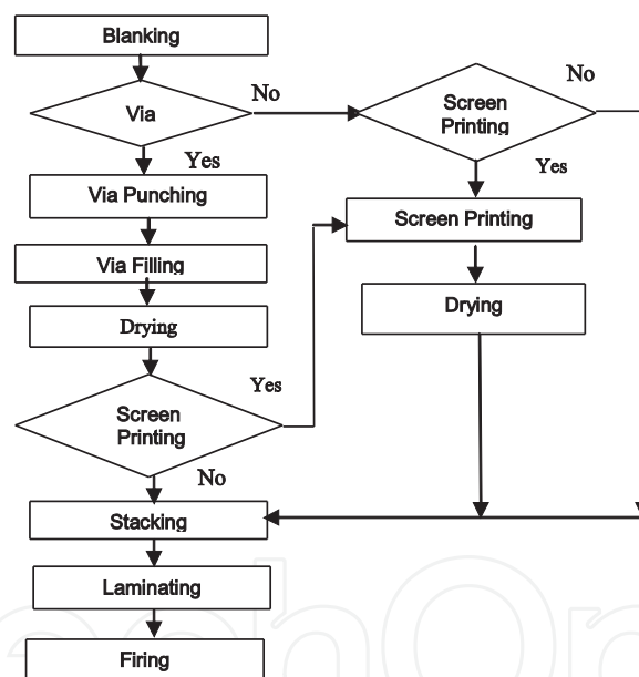
Figure 5. LTCC Multilayer Fabrication Process Flow.
