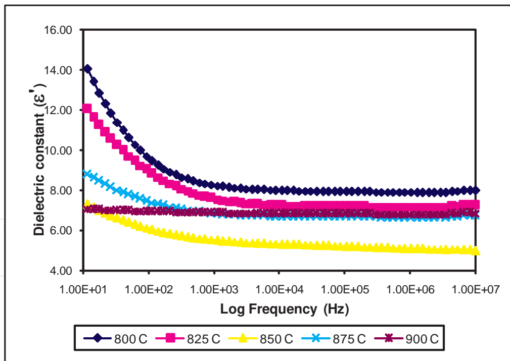
Figure 13. The variation of dielectric constant with frequency.
