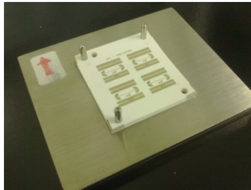
Figure 6. The manual stacker for collating and stacking process.
