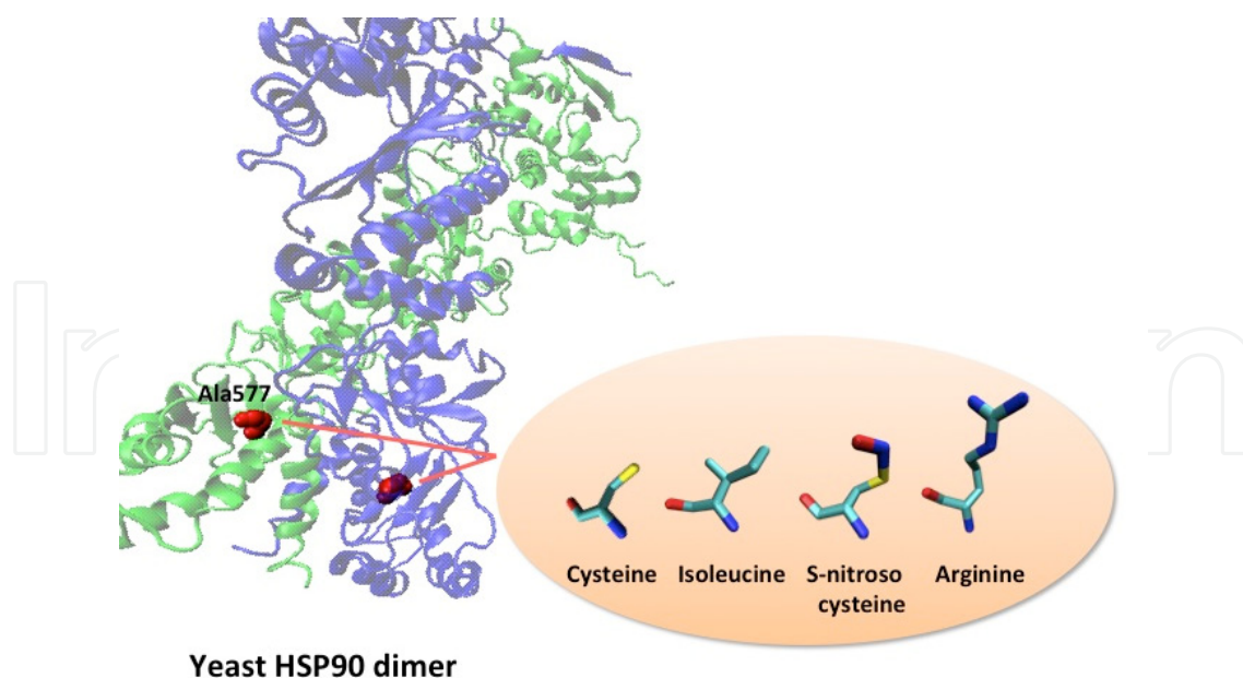
Fig. 4. Mimicking S-nitrosylation in an engineered regulatory site. Ribbon representation of X-ray crystal structure of the Yeast HSP90 dimer; native Ala 577 (left) and engineered variants at position 577 (right) are highlighted in red. Note that there are structural similarities between cysteine and the non-modifiable isoleucine and between S-nitrosocysteine and arginine. Structural coordinates were obtained from the Protein Databank (PDB code: 2CG9) Stick-models of residues were color-coded by atom type: carbon atoms are cyan, nitrogen atoms are blue, and oxygen atoms are red.
