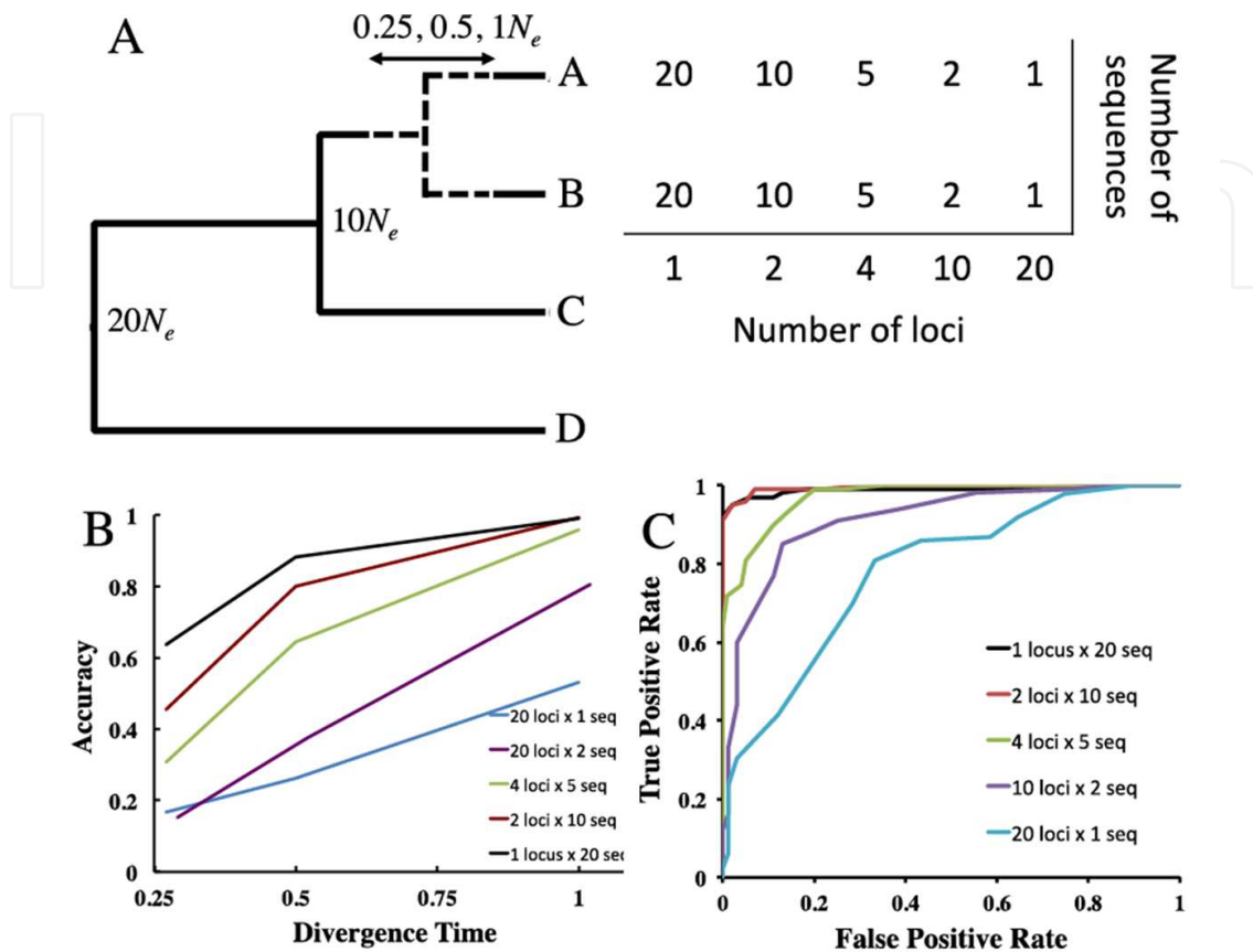
Figure 2. Simulation-based testing of the accuracy of BP&P to detect speciation between species A and B using five alternative sampling designs with the same sequencing effort and at three increasing divergence times (0.25, 0.5, and 1Ne) (A). Plot of accuracy and divergence time for each sampling design (B). ROC plot for each sampling design when divergence time = 0.5Ne (C).
