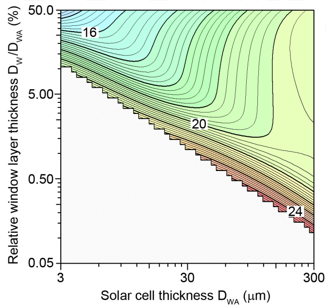
Figure 2. Dependence of Al 0.29 Ga 0.71 As/GaAs solar cell performance as a function of window and cell thickness
