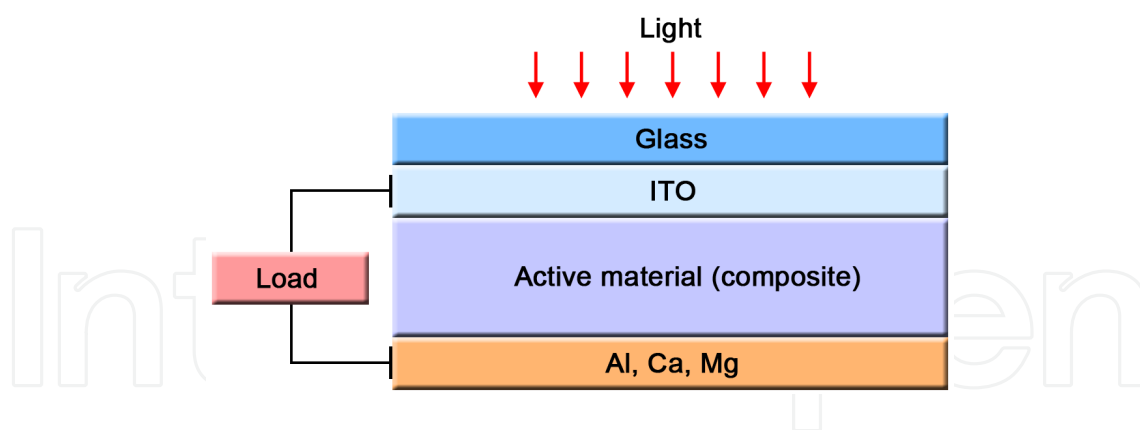
Figure 10. Photovoltaic solar cell: organic material sandwiched between two electrodes. The electrons are collected at the rear metal contact and the holes – at the front ITO contact.
