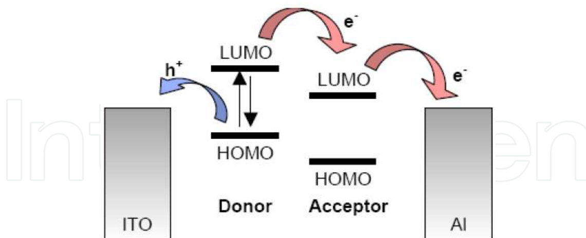
Figure 11. Exciton dissociation at the donor-acceptor interface
