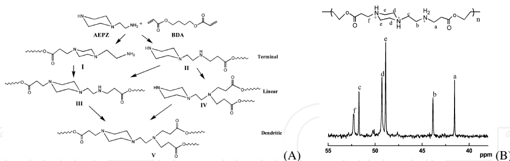
Figure 5. Possible routes of the Michael addition polymerization of trifunctional amine monomers and diacrylates (A) and the structure of poly(amino ester)s obtained and enlarged ^{13}\text{C} -NMR (INVGATE) spectrum of methylene carbons attached to the hydrochloride salts of amines in BDA-AEPZ (B). [Source from Ref. [50]].
