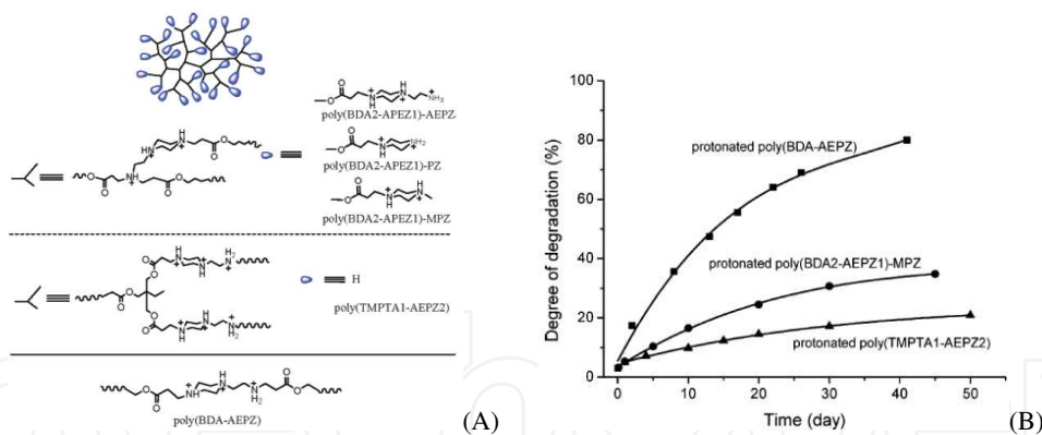
Figure 6. Structure of linear and hyperbranched poly(amino ester)s obtained via Michael addition polymerization of trifunctional amines with diacrylates and triacrylates (A) and comparison of the hydrolysis profiles of protonated hyperbranched poly(BDA2-AEPZ1)-MPZ, hyperbranched poly(TMPTA1-AEPZ2), and linear poly(BDA-AEPZ) in aqueous solutions (B). [Source from Ref. [51]].
