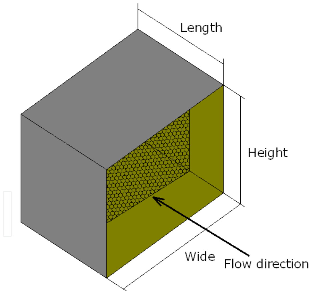
Figure 5. General layout of a settling chamber with a honeycomb layer.
