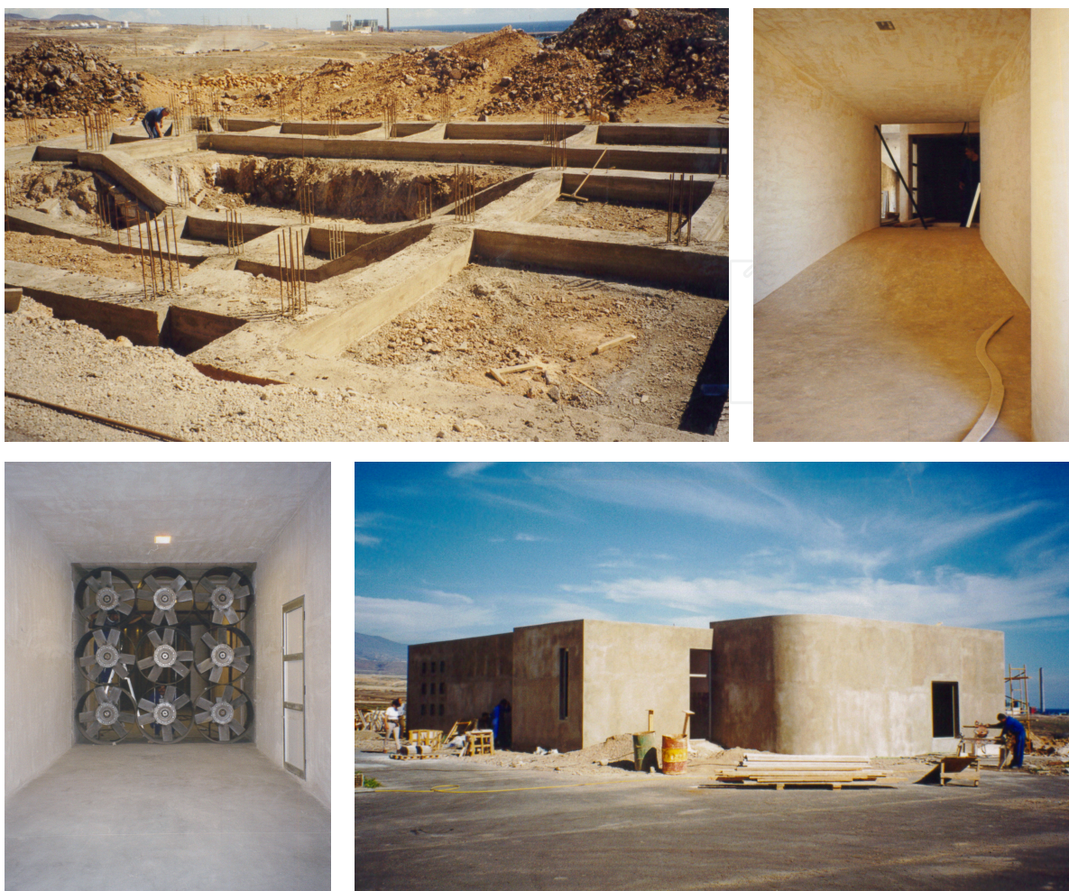
Figure 15. Photographic sequence of the construction of the ITER Low Speed Wind Tunnel. The top left picture shows the foundations, the top right the contraction, the bottom left the power plant and the bottom right a view from the outside almost at the end of the construction.
