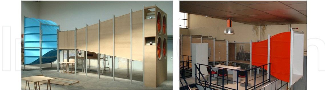
Figure 14. Research and education purpose wind tunnels built with wood panel and standard metallic profiles, with multi-fan power plant.
