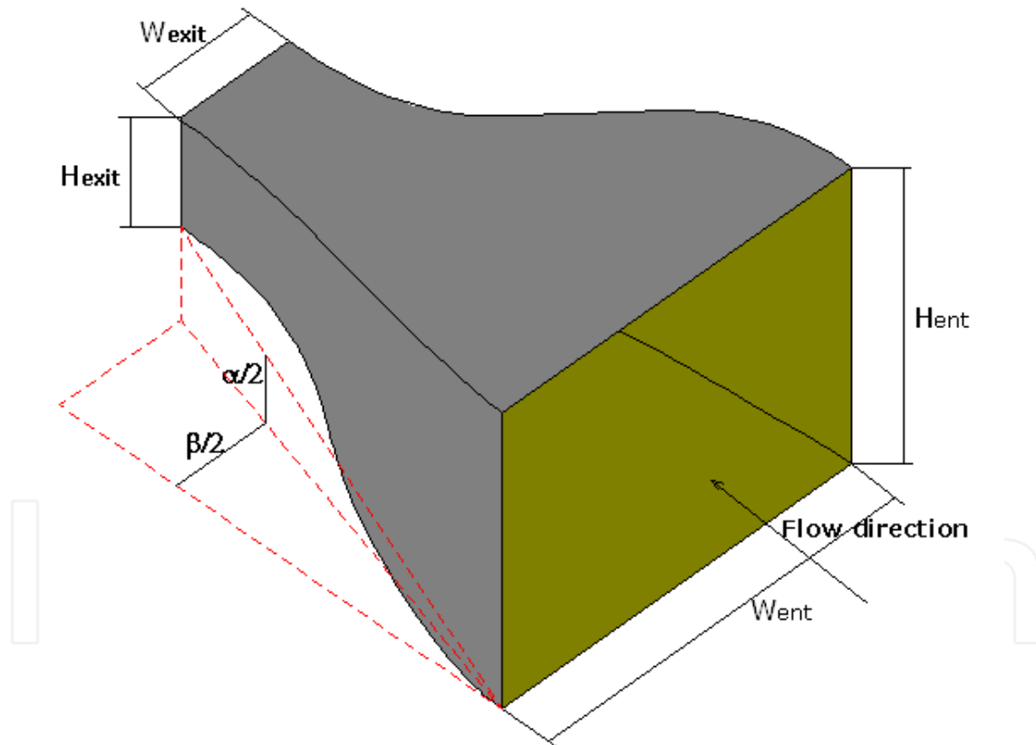
Figure 3. General layout of a three-dimensional wind tunnel contraction.
