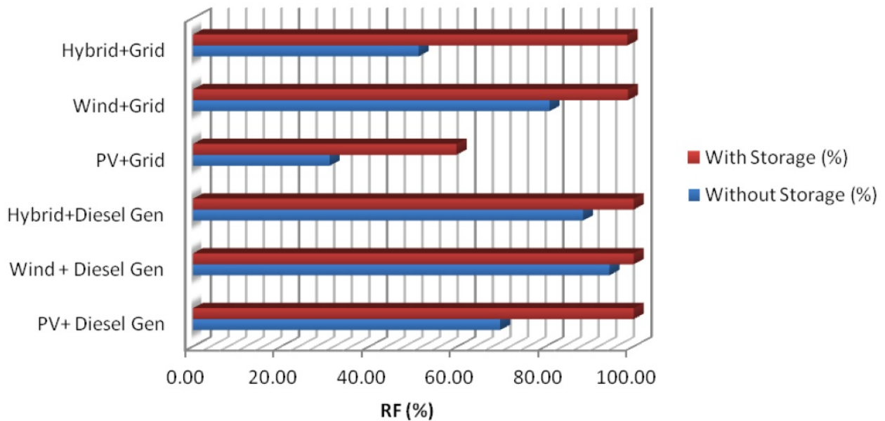
Figure 14. Renewable fraction (RF) in different cases
