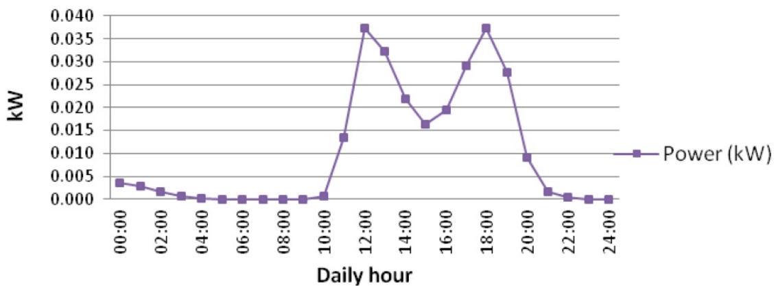
Figure 7. Energy converted per m² area at 40m height wind speed in Rockhampton
