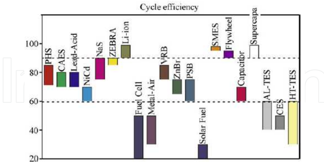
Figure 18. Cycle efficiency of EES systems. [69]
