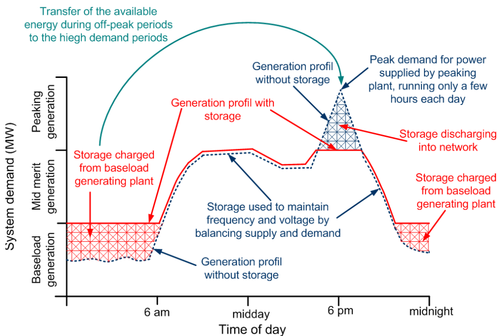
Figure 1. Fundamental idea of the energy storage [55]
