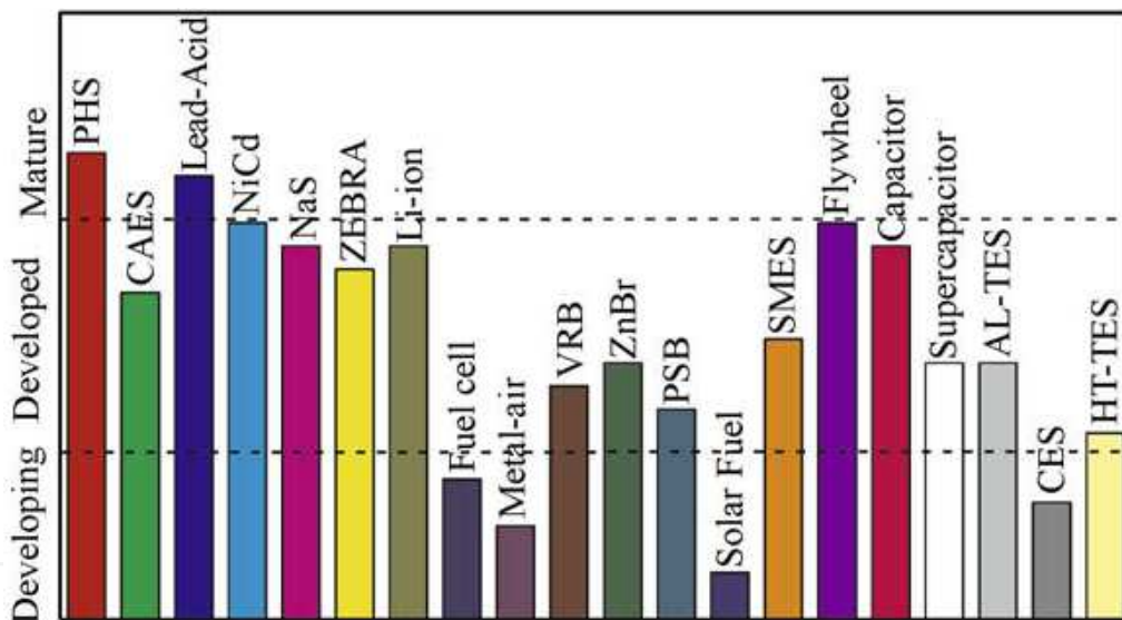
Figure 17. Technical maturity of EES systems [69]
