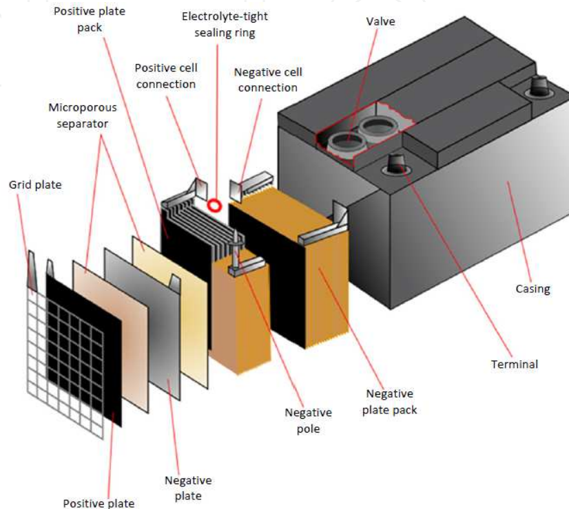
Figure 13. Structure of a lead-acid battery [86]
