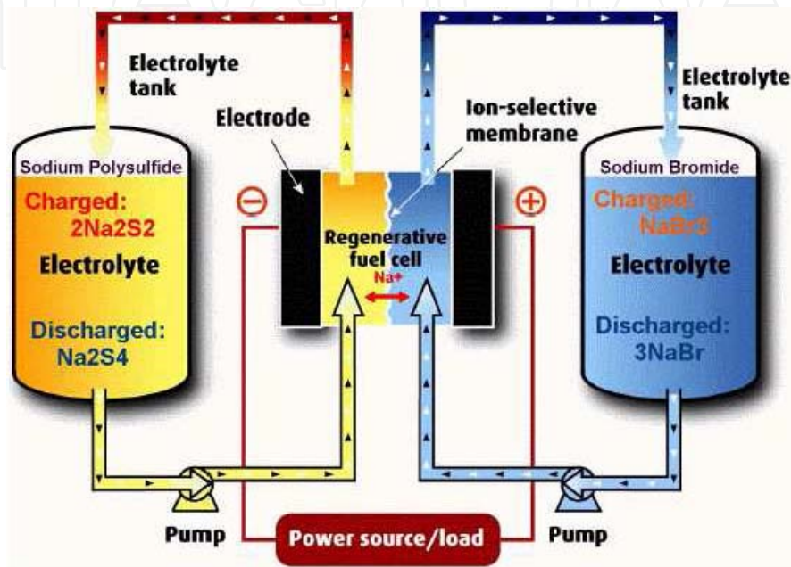
Figure 14. Illustration of a flow-battery
