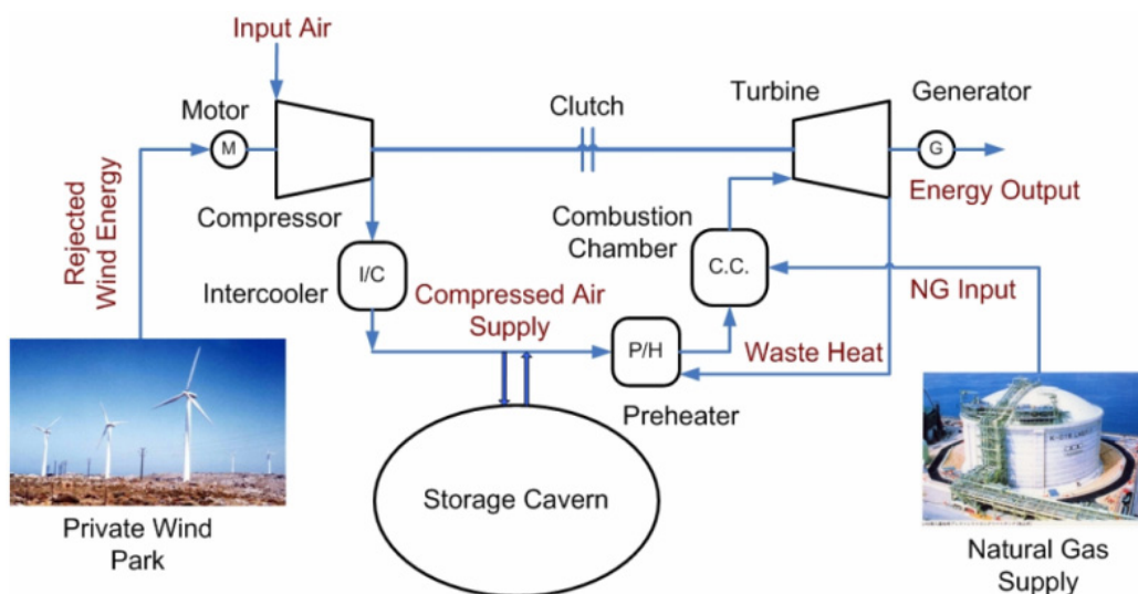
Figure 16. Illustration of compressed-air energy storage
