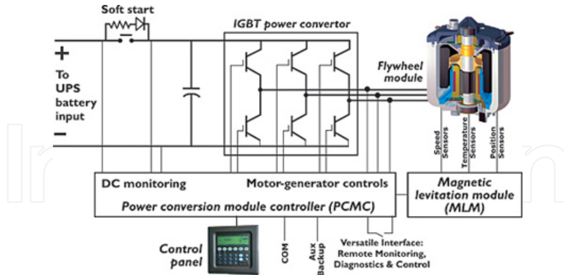
Figure 15. Flywheel energy accumulators [89]
