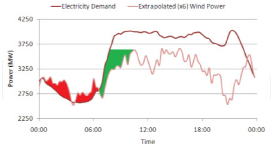
Figure 5. Integration of extrapolated (x6) wind power using energy storage on the Irish electricity grid [58]
