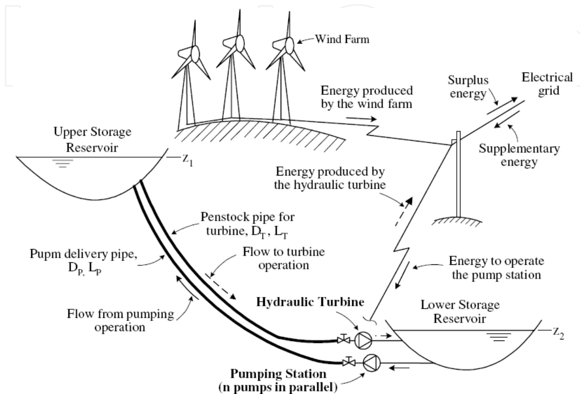
Figure 12. Wind-Pumped hydro energy storage hybrid system [69].
