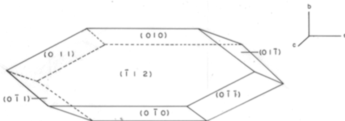
Figure 3. Morphology representation of NTF crystal
