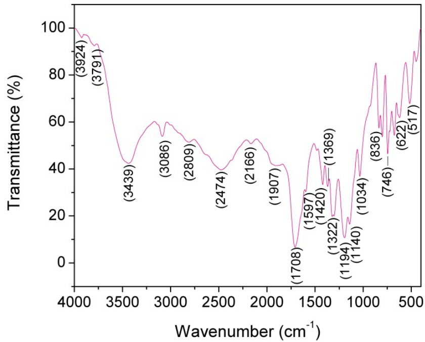
Figure 14. FTIR spectrum of NTF
