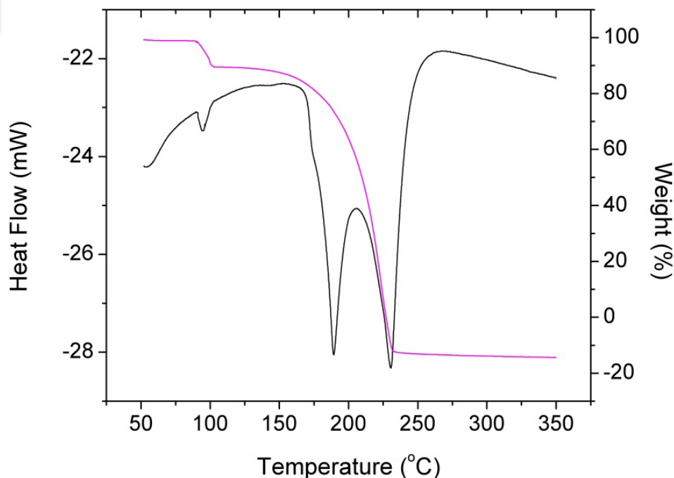
Figure 12. TGA-DTA curves of NNM
