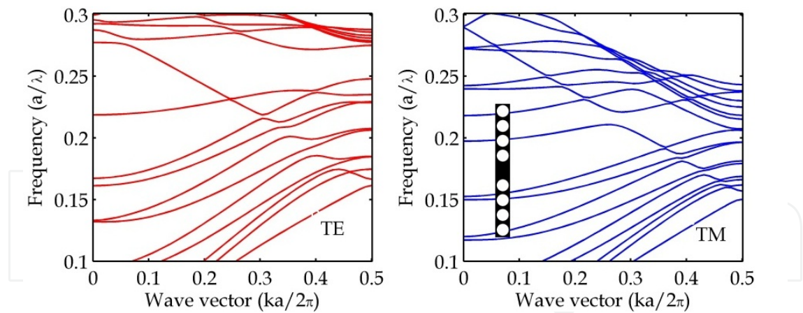
Figure 6. Dispersion curves of line defect square lattice PhCW. The inset is the 1 \times 9a supercell used in PWE calculations. The parameters of the PhCW are chosen as follow: permittivity of high and low index materials are 12.96 and 1, respectively and the radius of air holes is r=0.40a .
