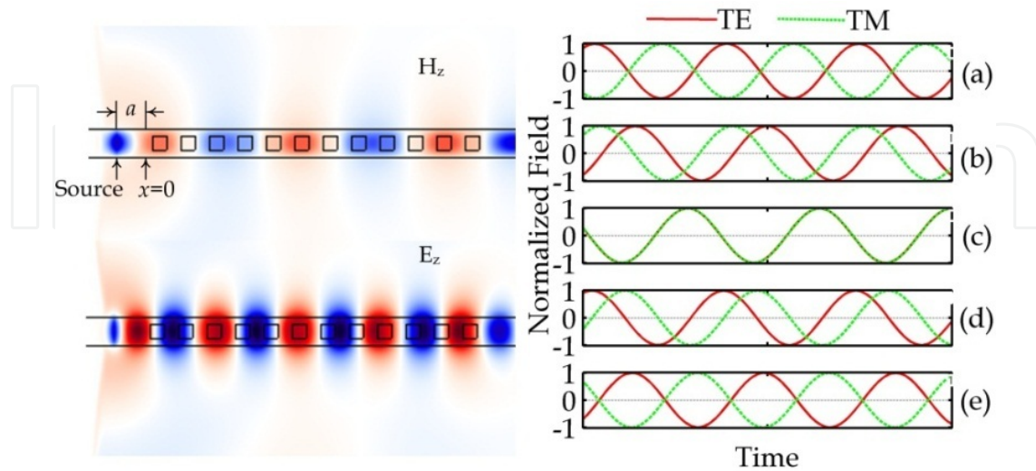
Figure 17. [Left] Snapshots of EM fields at frequency of 0.14 a/\lambda for TE ( H_z ) and TM ( E_z ) polarizations. [Right] Normalized EM field variations with time for TE and TM modes with same frequency of 0.14 a/\lambda but at different space locations of 2.9a (a), 4.45a (b), 6.4a (c), 7.9a (d), and 89.6a (e), respectively. [11]
