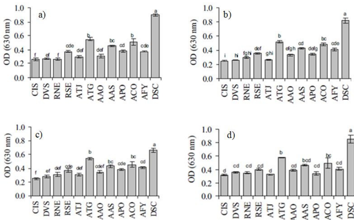
Figure 3. Effect of different fructans on the growth of a) B. adolescentis ; b) B. infantis ; c) L. paracasei and d) L. rhamnosus incubated anaerobically at 37°C in the presence of 10 g of fructan/L. OD, Optical density; CIS, Cichorium intybus ; DVS, Dahlia variabilis ; RNE, Raftiline; RSE, Raftilose; ATJ, A. tequilana Jalisco; ATG, A. tequilana Guanajuato; AAO, A. angustifolia Oaxaca; AAS, A. angustifolia Sonora; APO, A. potatorum Oaxaca; ACO, A. cantala Oaxaca; AFY, A. fourcroydes Yucatán; DSC, Dasylirion sp. Chihuahua.
