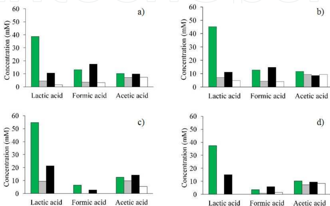
Figure 4. Concentration of short chain fatty acids generated by bifidobacteria and lactobacilli from the fermentation of Dasyilirion sp. (DSC; ■), Raftilose (RSE; ■), A. tequilana GTO. (ATG; ■) and Raftiline (RNE; □). a) B. adolescentis ; b) B. infantis ; c) L. paracasei and d) L. rhamnosus .
