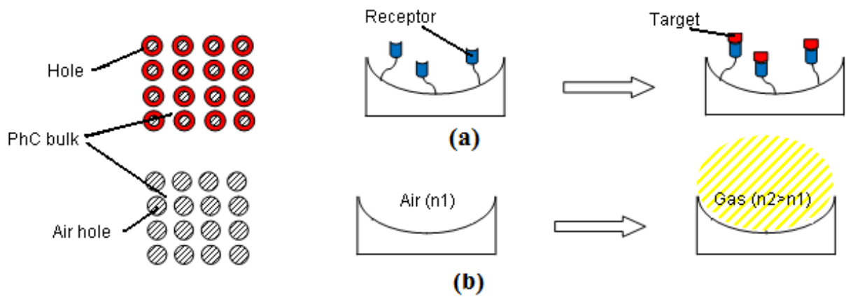
Figure 1. a) Surface sensing and (b) homogeneous sensing. Probe molecules (blue) are deposited on hole surfaces and target molecules (red) are captured by receptors forming an adlayer on the sensor surface.
