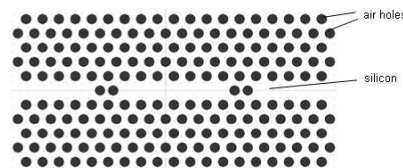
Figure 18. Schematic of L6 cavity to generate Raman effect.
