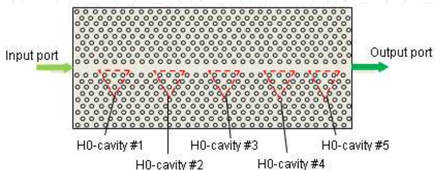
Figure 8. Array of H0 resonant cavities.
