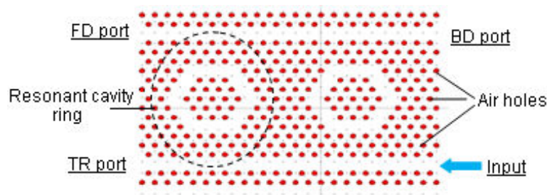
Figure 19. Schematic of DNR channel drop filter.
