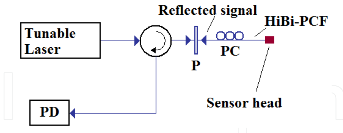
Figure 29. Schematic of the measurement setup of the magnetic field sensor.
