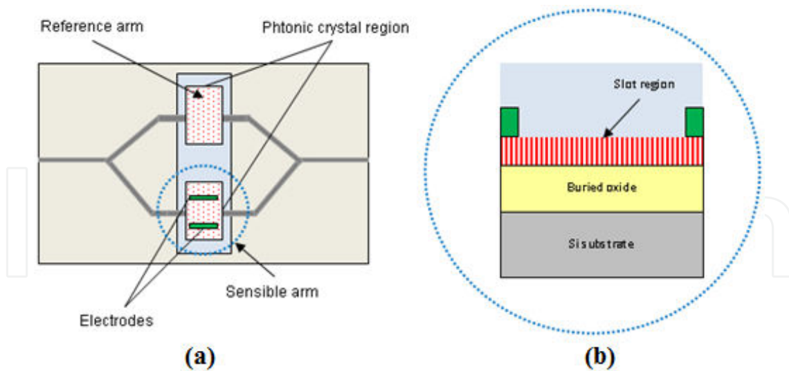
Figure 14. MZI with slot Photonic Crystal waveguide (a) and cross-sectional view (b).
