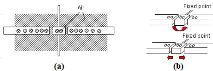
Figure 22. Schematic of the torsion PhC-based sensor (a) and operative configurations (b): right torsional (top) and flexural (bottom) movements of central sensor element.
