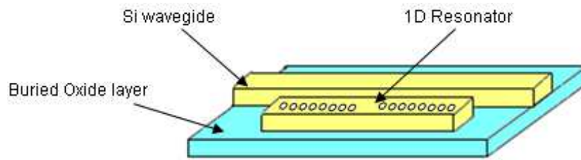
Figure 9. 1D-photonic crystal microcavity.
