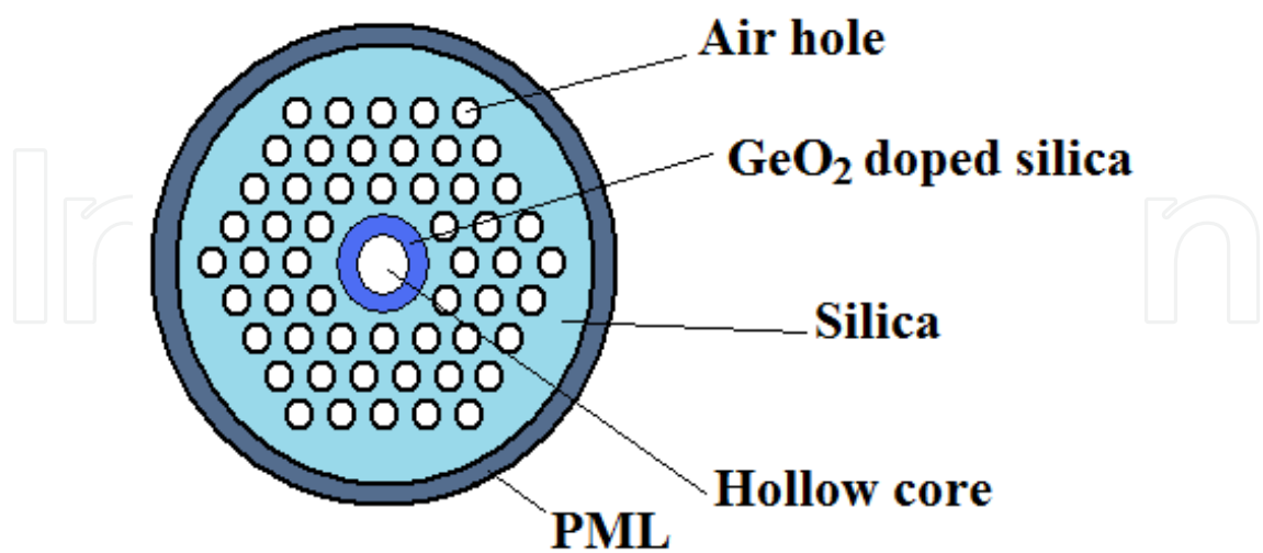
Figure 34. Cross section of the PCF characterized by a hollow GeO 2 -doped high index ring defect.
