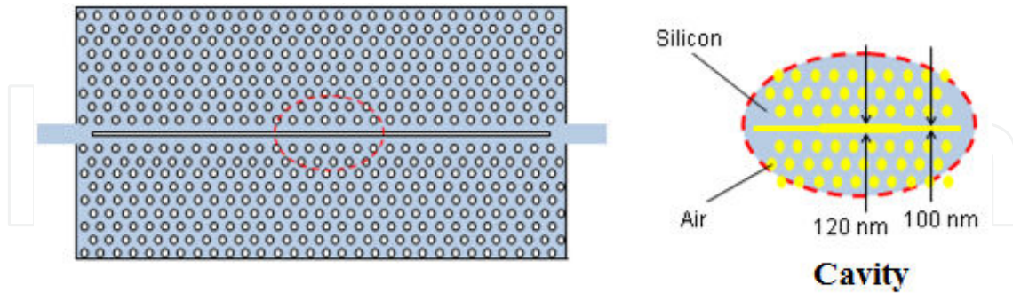
Figure 4. Air-slot PhC cavity with zoom of slit in the slot.
