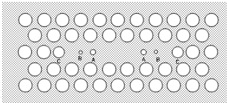
Figure 3. Zoom of cavity region of L7 cavity.
