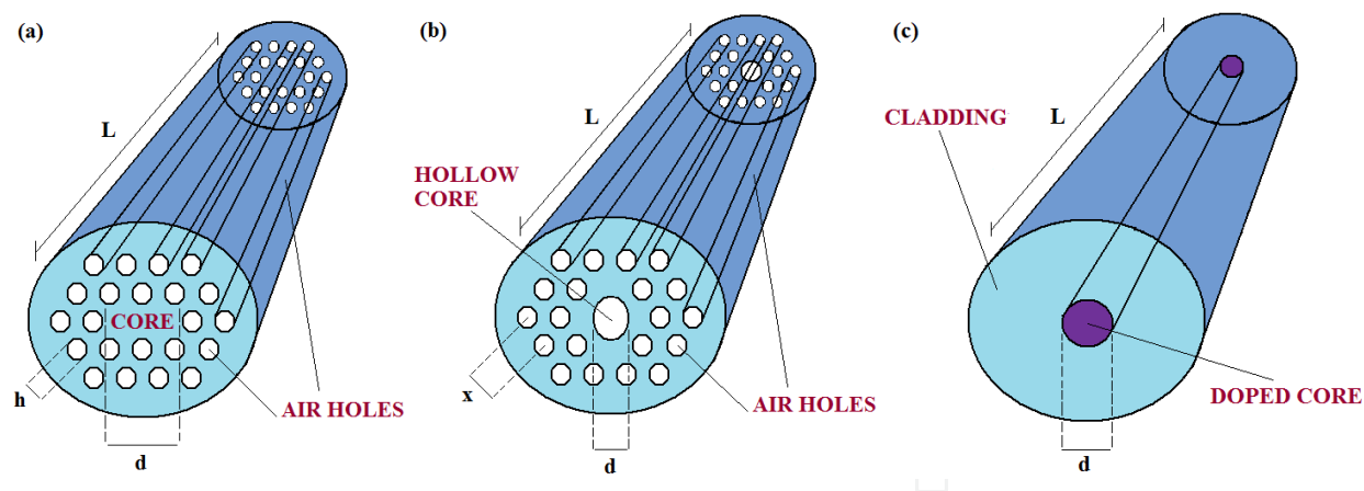
Figure 24. Schematic of (a) solid core PCF, (b) hollow core PCF, and (c) conventional SMF.
