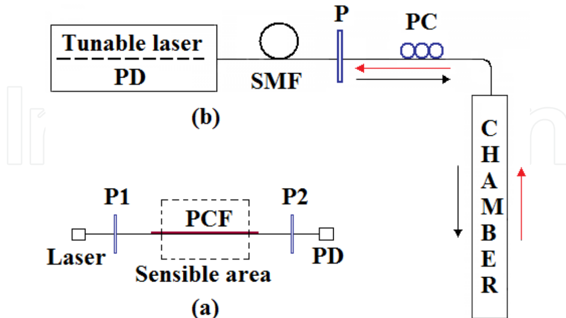
Figure 28. (a) Unidirectional and (b) bidirectional polarimetric measurement scheme used for pressure sensing.
