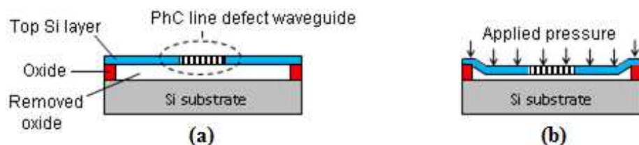
Figure 21. Sensor at rest (a) and sensor with applied pressure (b).
