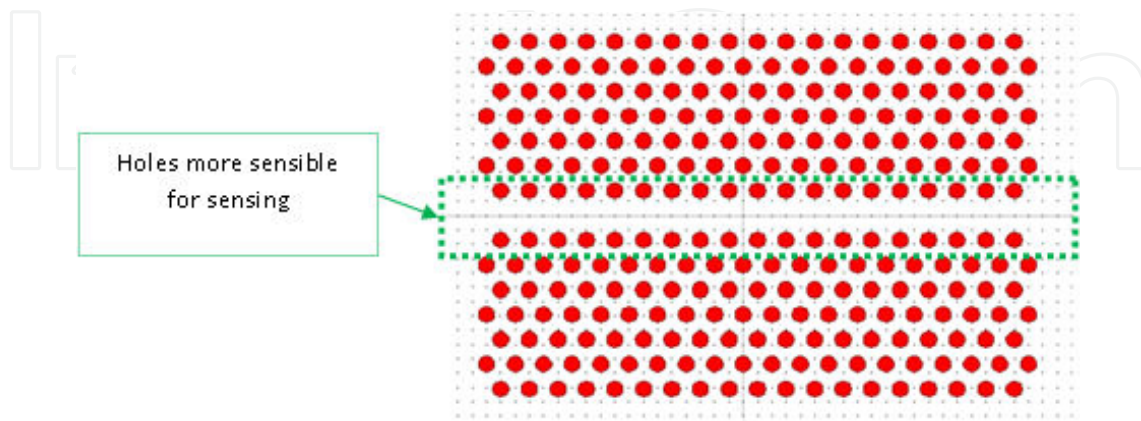
Figure 12. Photonic crystal waveguide sensor with sensible holes.
