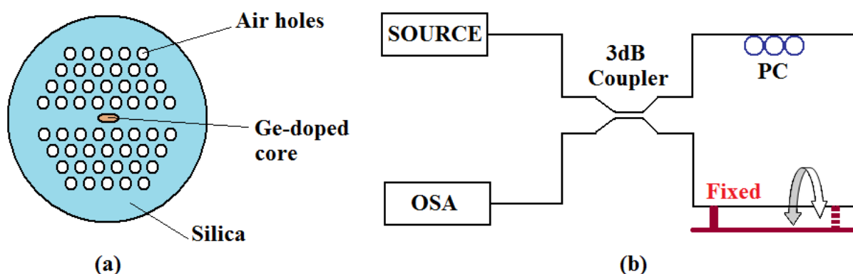
Figure 25. Schematics of the (a) Ge-doped PCF cross-section and (b) of the experimental setup for torsion sensing.
