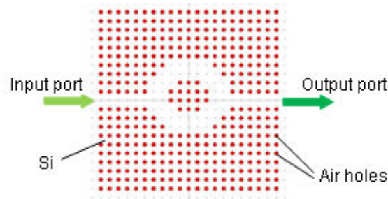
Figure 5. Schematic structure of sensor for seawater sensing.
