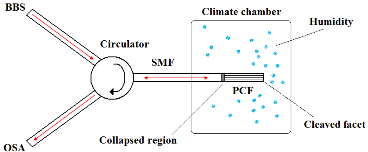
Figure 32. Schematic of the humidity sensor based on PCF interferometer.
