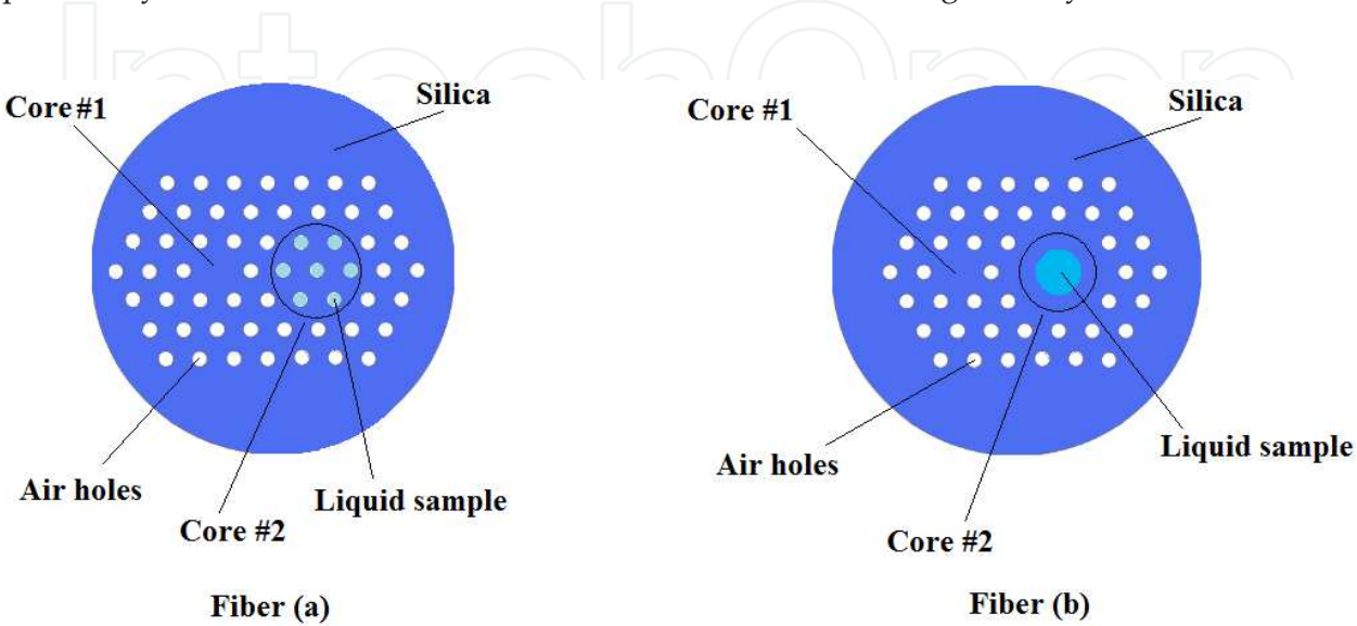
Figure 33. Cross sections of the analyte-filled micro-structured dual-core PCF (a), and dual-core PCF with an enlarge analyte-filled hole (b).
