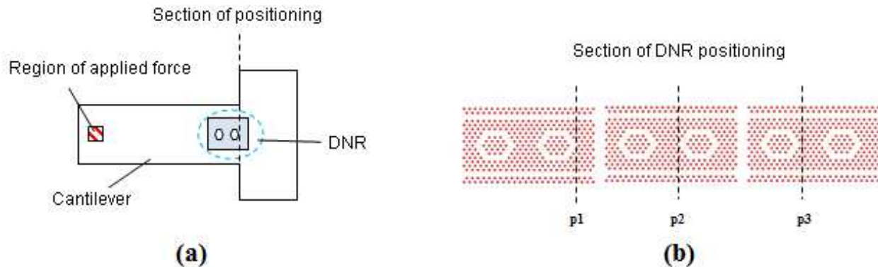
Figure 20. Cantilever architecture (a) and different positioning of DNR on cantilever (b).
