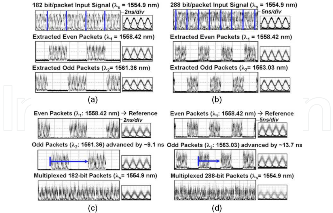
Figure 23. Temporal waveforms of time-slot exchange of 40-Gbit/s odd and even packets with two variable packet lengths. (a)(c) 182 bits/packet. (b)(d) 288 bits/packet.
