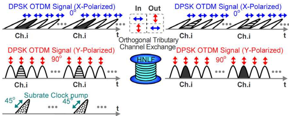
Figure 16. Concept and principle of Kerr effect-based orthogonal tributary channel exchange of a pol-muxed DPSK OTDM signal.
