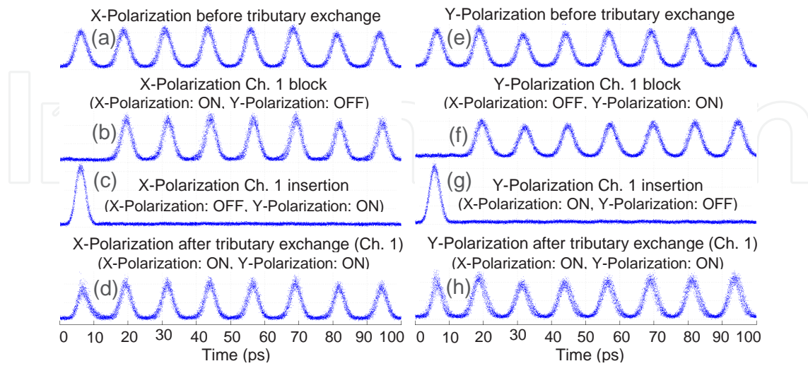
Figure 17. Eye diagrams of orthogonal tributary channel (Ch. 1) exchange of a 160-Gbit/s pol-muxed DPSK OTDM signal.
