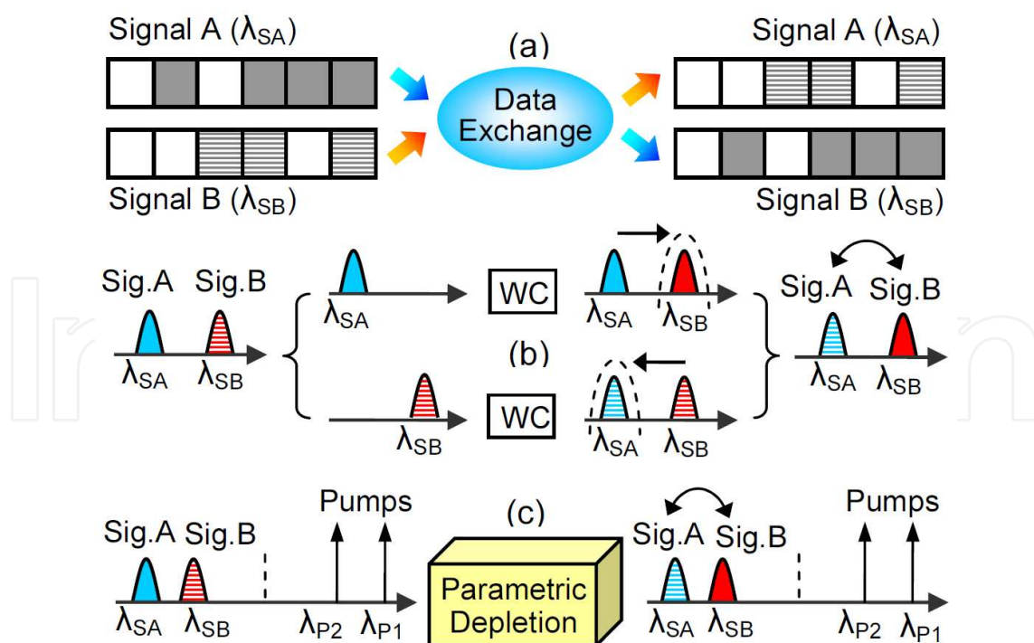
Figure 2. (a) Concept of data exchange in the wavelength domain. (b) Data exchange by two separate wavelength converters (WCs). (c) An example of data exchange by signal depletion and wavelength conversion in a single nonlinear device.
