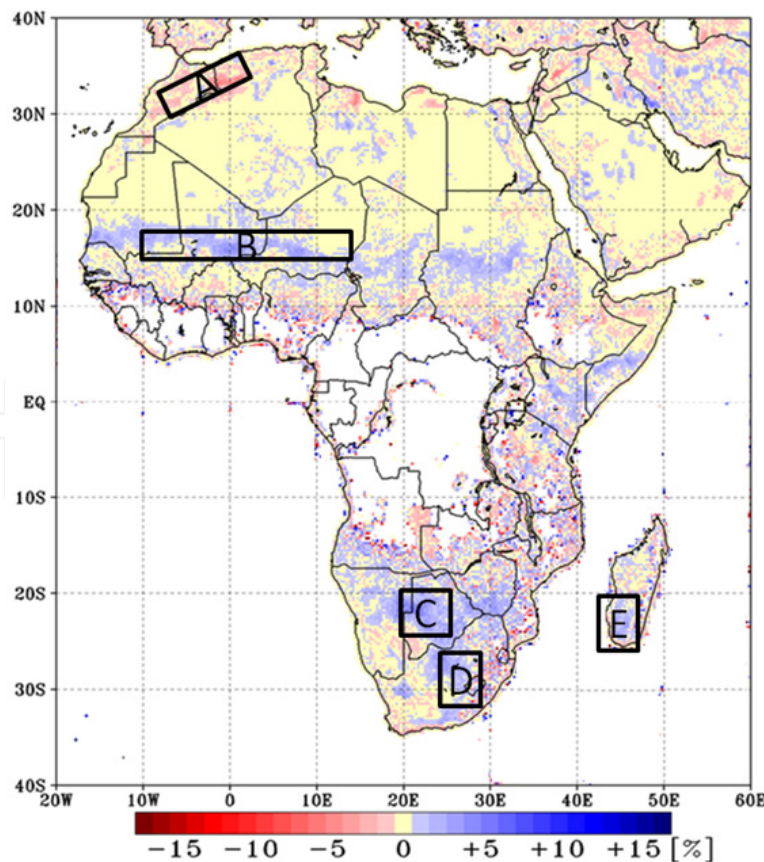
Figure 2. Difference between two decade-average summer soil moisture (%)
