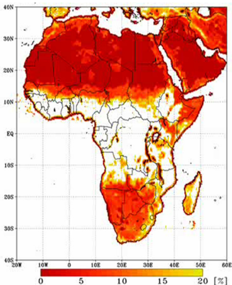
Figure 1. Retrieved montly averaged soil moisture from SSM/I
