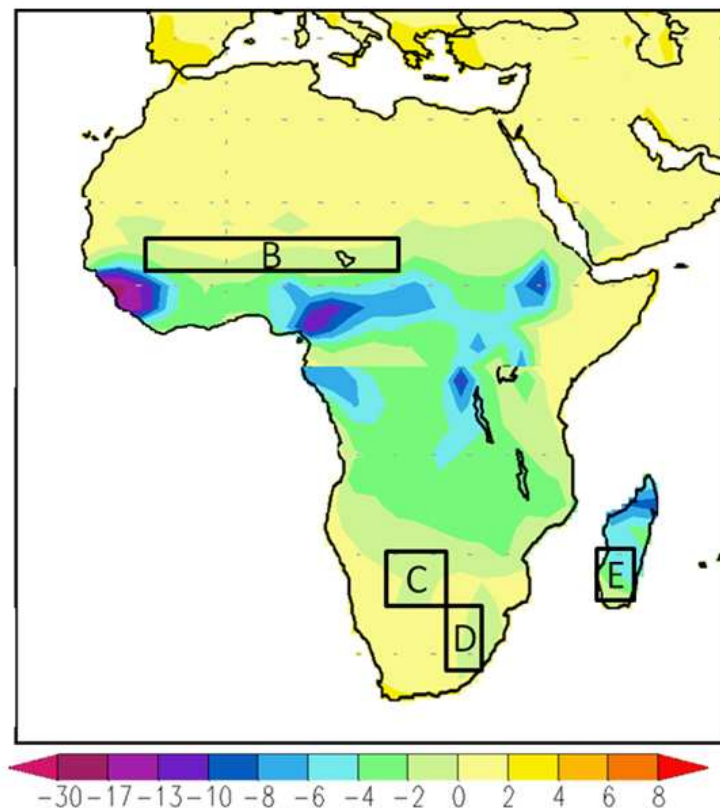
Figure 7. 20 years averaged ( E-P ) from ERA-40 (unit: mm)
