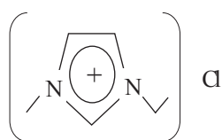
Figure 1. Chemical structure of 1-ethyl-3-methylimidazolium chloride ([C2mim][Cl])
