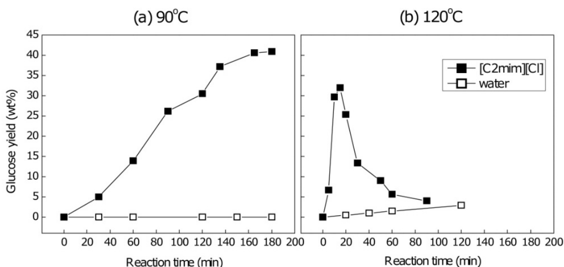
Figure 16. Comparisons of glucose yield from cellulose treated in the reaction system of [C2mim][Cl] and water as solvent at (a) 90 °C and (b) 120 °C with 1.5 wt% sulfuric acid
