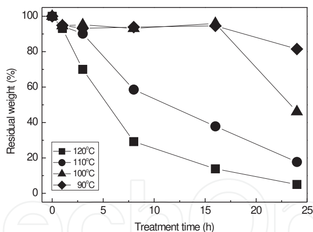
Figure 2. Changes in residual weight of Japanese beech after [C2mim][Cl] treatment at various temperatures
