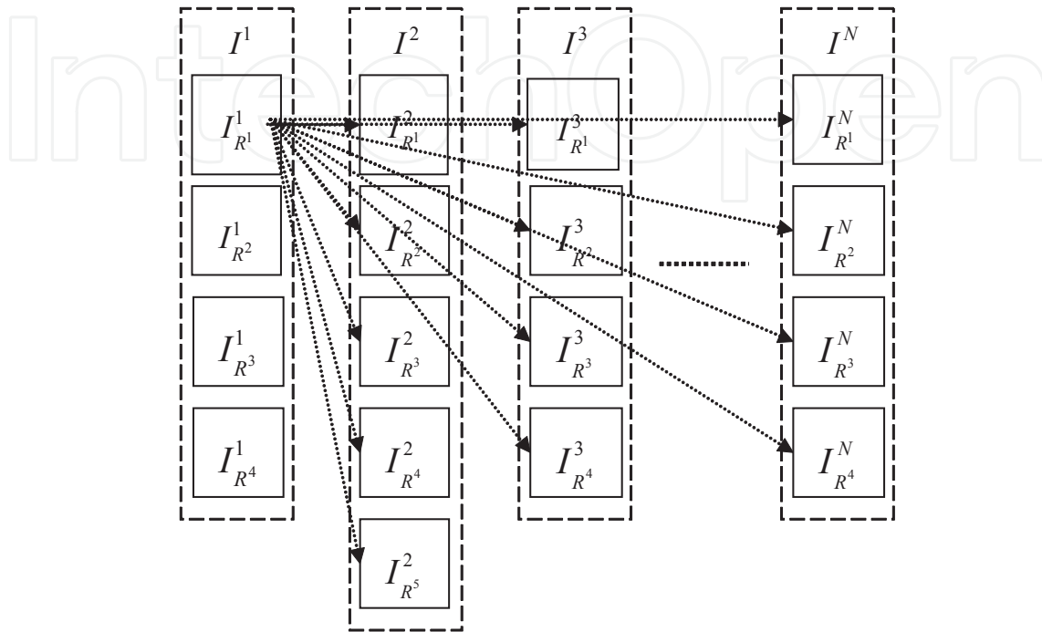
Figure 6. The similarity matching for region pairs.
