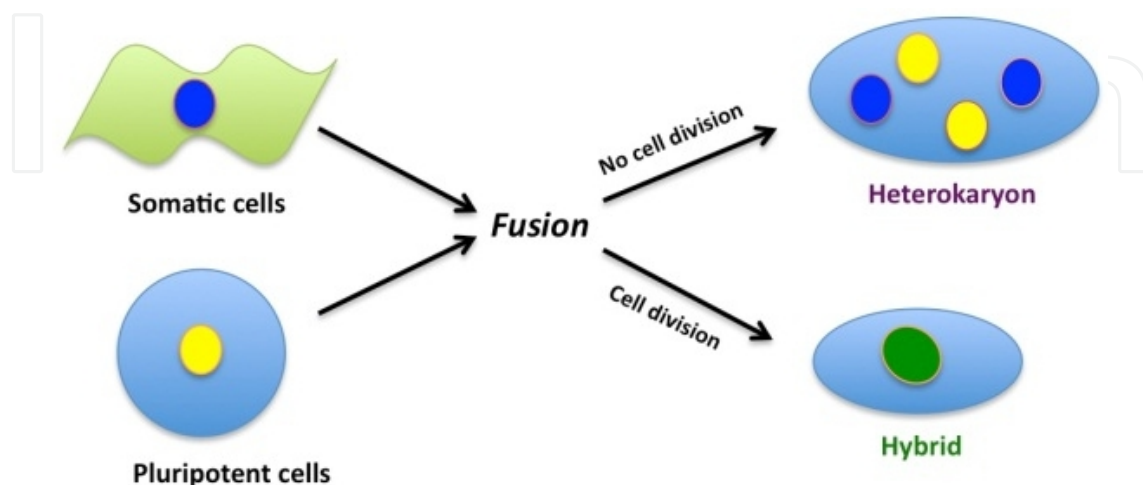
Figure 2. Cell fusion
