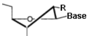
Figure 7. C2'-endo (DNA-like) conformation of ribose with the substituent (R) in 2'-position.
