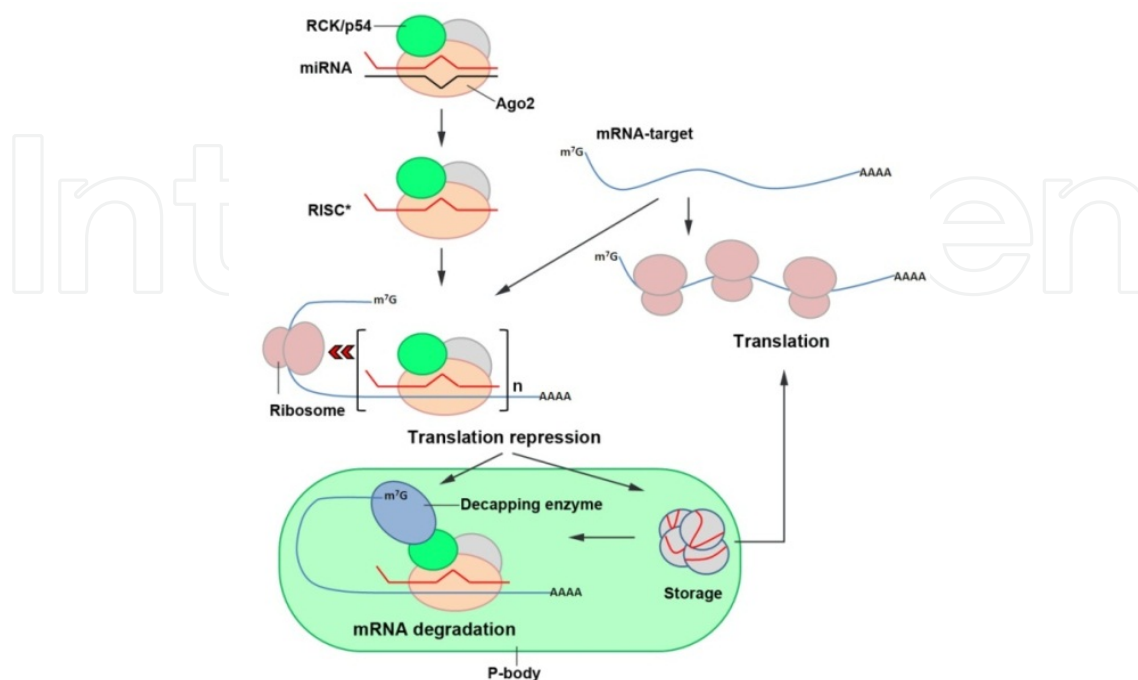
Figure 4. Scheme of RNAi with the “bypass” route of RISC* assembly (miRNA-like action). RISC* binds with mRNA-target ( n is equal 1, if the antisense strand is fully complementary to mRNA) [10].
