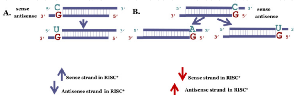
Figure 10. The scheme of the experiment described in 38 . A. Substitution at the 5'-end of the sense strand of anti- F.luciferase siRNA. B. Substitution at the 3'-end of the sense strand (left) or at the 5'-end of the antisense strand (right) of anti- sod1 siRNA.
