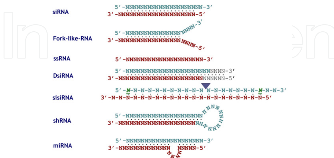
Figure 9. Structural repertoire of siRNA. The triangle indicates single stranded nick.
