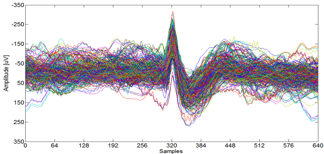
Figure 8. Representation of the selected events for the choice of the Wavelet function to be used in the filtering of signals.
