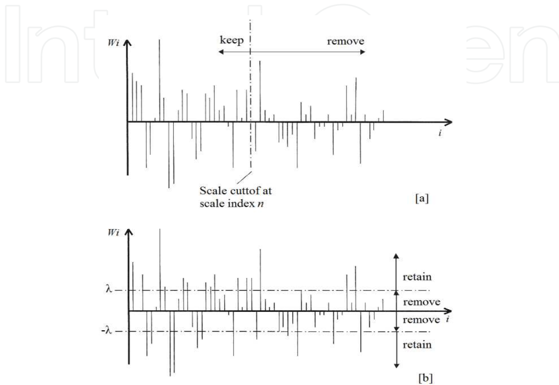
Figure 3. Representation of some ways to suppress coefficients in the Wavelet domain used to process a signal.
