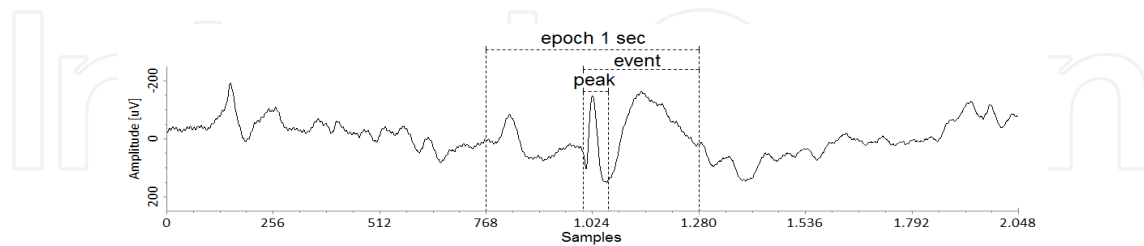
Figure 10. Representation of the categories defined for the analysis of the Wavelet functions.
