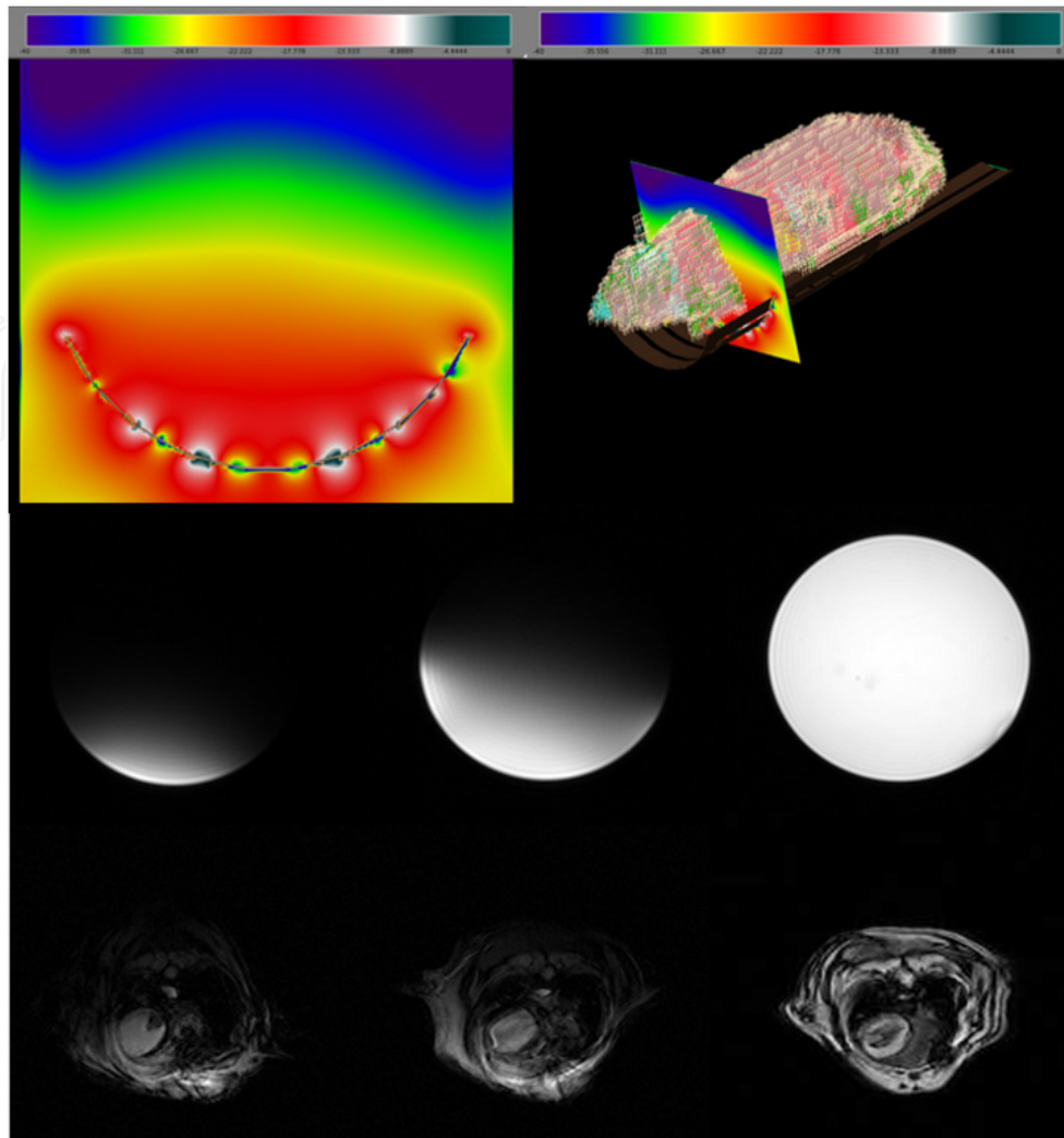
Figure 7. (Top, Left) Mouse XFDTD B 1 -field simulation of a four-spiral cylindrical coil under loaded conditions with a mouse computational model (top, right) [color bar varies between 0 – -40 dB];(Bottom) Flat, cylindrical spiral, and birdcage axial phantom response using conventional SPGR pulse sequence acquisitions and corresponding cardiac MRI from each of the three coils in mice post-mortem showing improved performance by the birdcage coil. [This figure originally appeared in Constantinides C et al., Intercomparison of performance of RF Coil Geometries for High Field Mouse Cardiac MRI. Concepts of Magnetic Resonance Part A, 38A(5):236-252, 2011, DOI 10.1002/cmr.a.20225, reproduced with permission from Wiley Publications].
