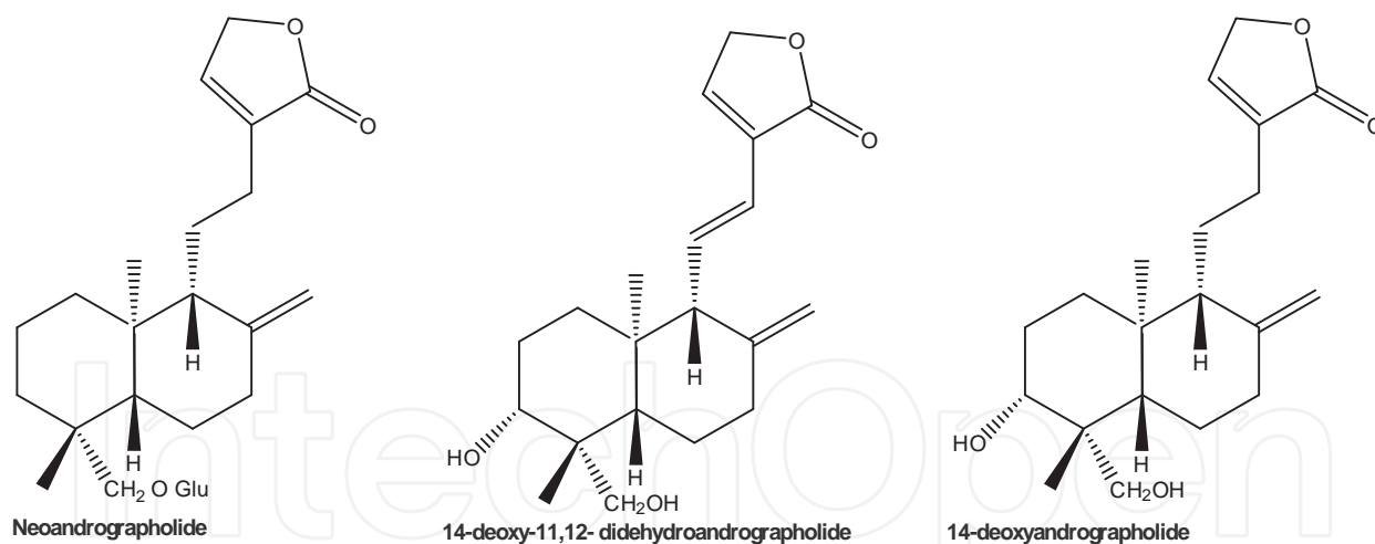
Figure 2. Chemical structure of minor labdane diterpenes isolated from Andrographis paniculata .
