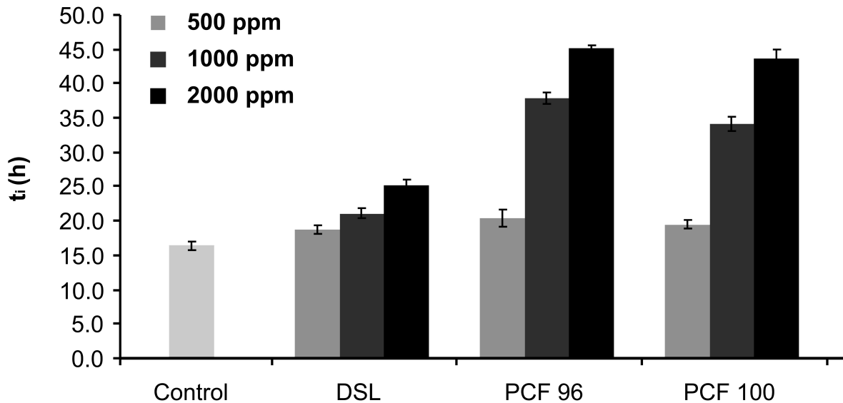
Figure 3. Induction times ( t_i ) of refined sunflower oil (control) added with different concentrations of modified sunflower lecithins (Rancimat Mod 679, Metrohm). Mean values ( n = 3 ) \pm sd
