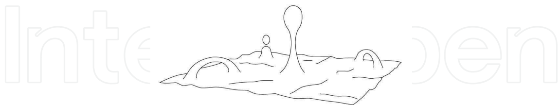
Figure 2. Space-time foam: some of the baby universes may branch off from the parent space-time.
