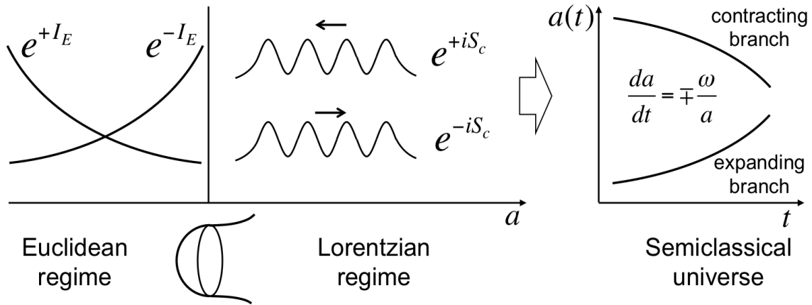
Figure 3. Boundary conditions of the universe.
