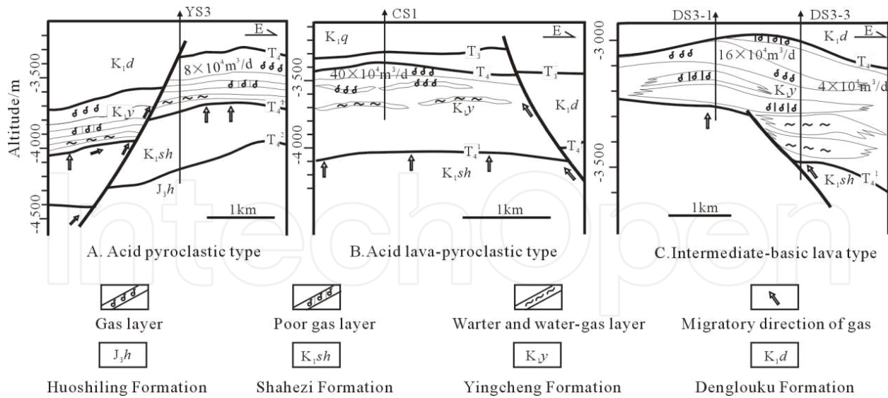
Figure 10. Forming pattern of gas pools of volcanic edifices in the Songliao Basin
