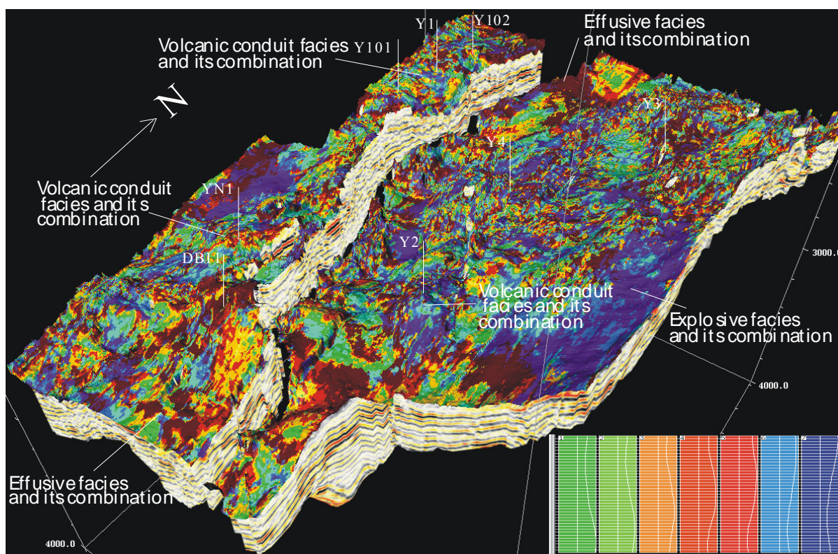
Figure 7. Waveform classification (seismic facies) map of volcanic rocks of the upper Yingcheng Formation in the YYT work area
