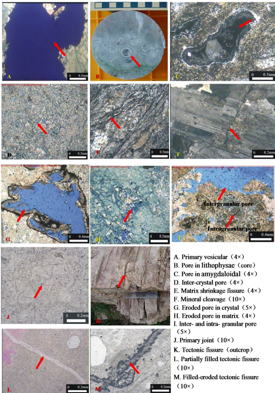
Figure 4. Volcanic reservoir space types
