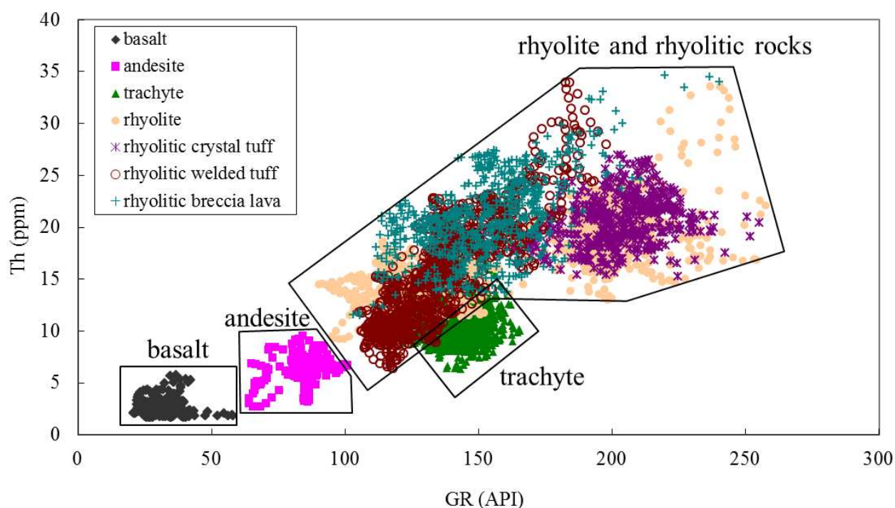
Figure 5. Cross-plot of GR versus Th for lithological identification of volcanic rocks of the Lower Cretaceous Yingcheng Formation in the Xujiaweizi depression, Songliao Basin, China
