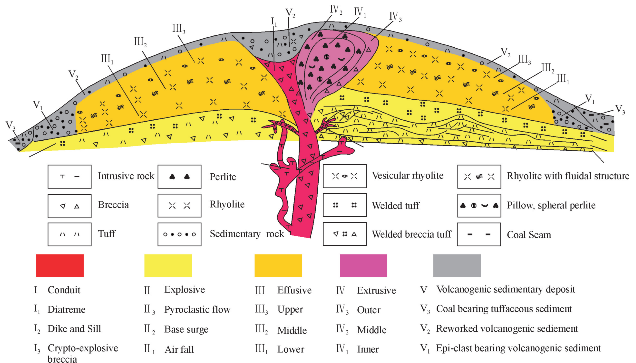
Figure 3. Model of the facies of Mesozoic acidic volcanic rocks in the Songliao Basin, China
