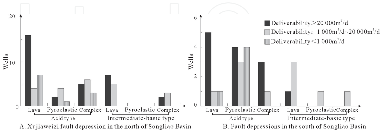
Figure 9. The relationship between hydrocarbon accumulations and volcanic edifices in the Songliao basin
