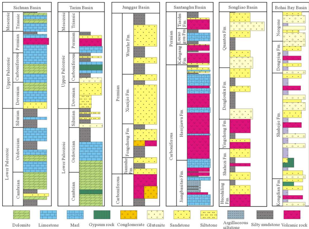
Figure 8. Source-reservoir-cap assemblages of the volcanic oil and gas accumulations in main petroliferous basins of China (Zou et al. [81])
