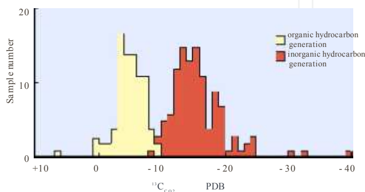
Figure 2. Organic and inorganic origin \delta^{13}\text{C}_{\text{CO}_2} frequency (Dai [62, 65])
