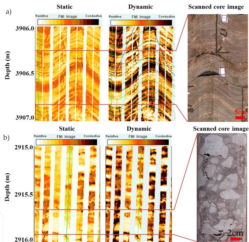
Figure 6. Typical lithological structures on FMI logging image. a) Flow bandings of extrusive rhyolite; b) Volcanic breccia structure of explosive facies.
