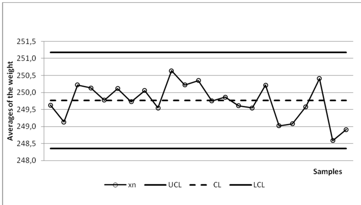
Figure 6. Chart of Average ( \bar{x} ) (without the 23th subgroup)
