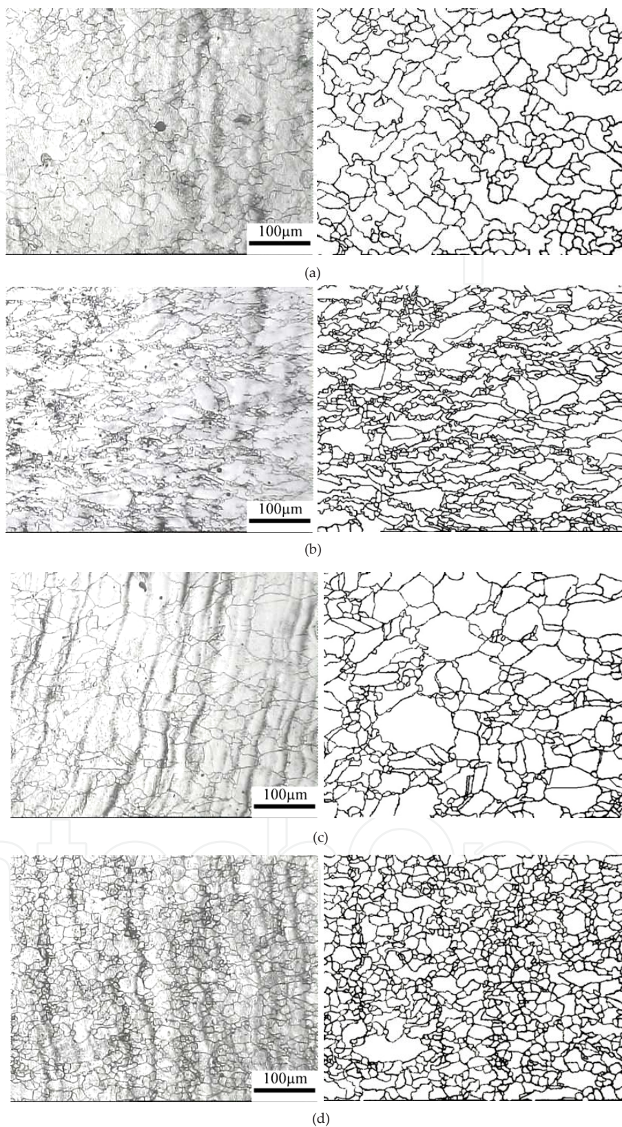
Figure 14. Optical microstructures of 42CrMo high-strength steel at a fixed true strain of 0.9, a fixed temperature of 1123 K and different strain rates: (a) 0.01 \text{ s}^{-1} , (b) 0.1 \text{ s}^{-1} , (c) 1 \text{ s}^{-1} , (d) 10 \text{ s}^{-1} .
