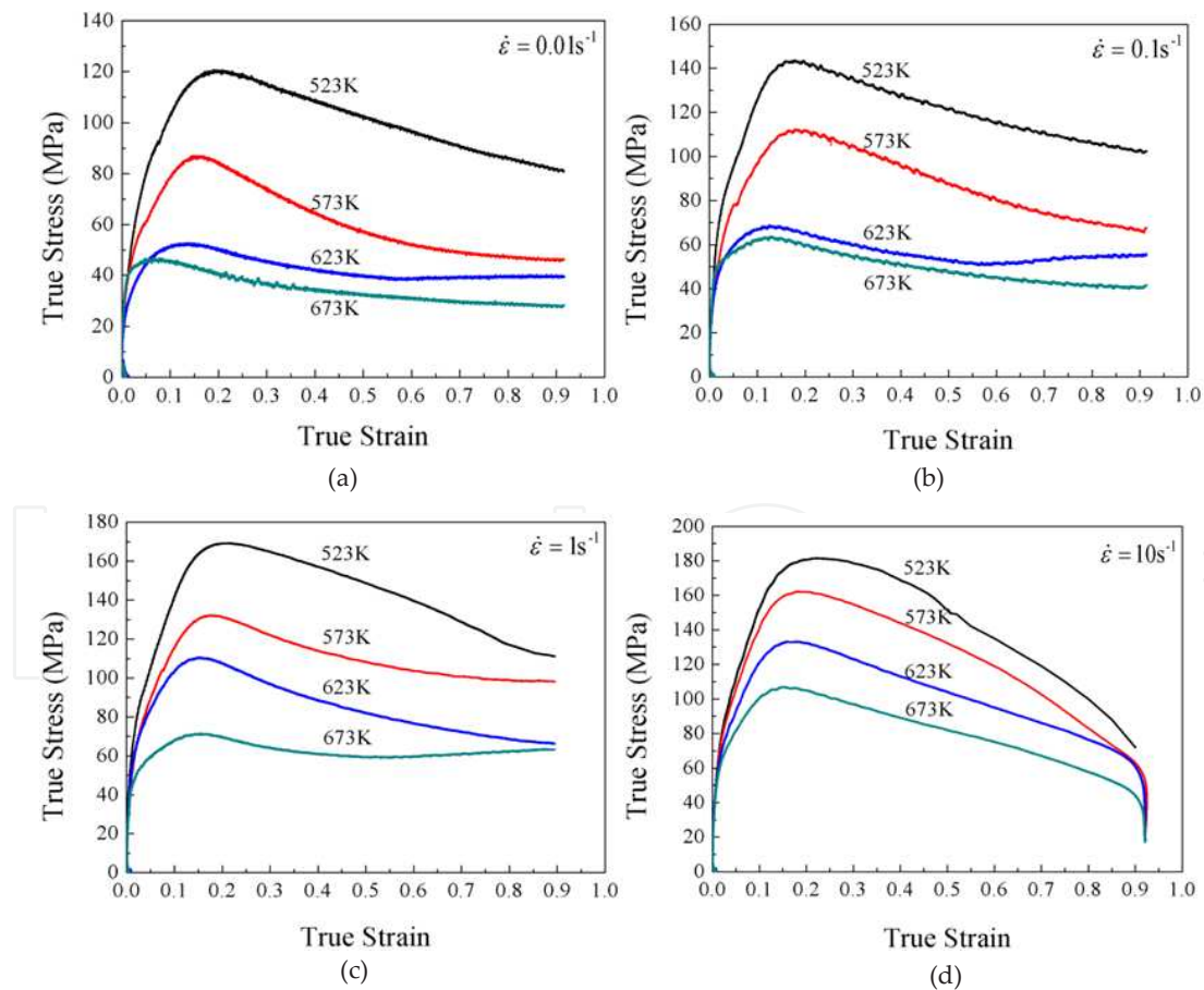
Figure 4. True stress-strain curves of as-cast AZ80 magnesium alloy obtained by Gleeble 1500 under different deformation temperatures with strain rates (a) 0.01 s -1 , (b) 0.1 s -1 , (c) 1 s -1 , (d) 10 s -1 .
