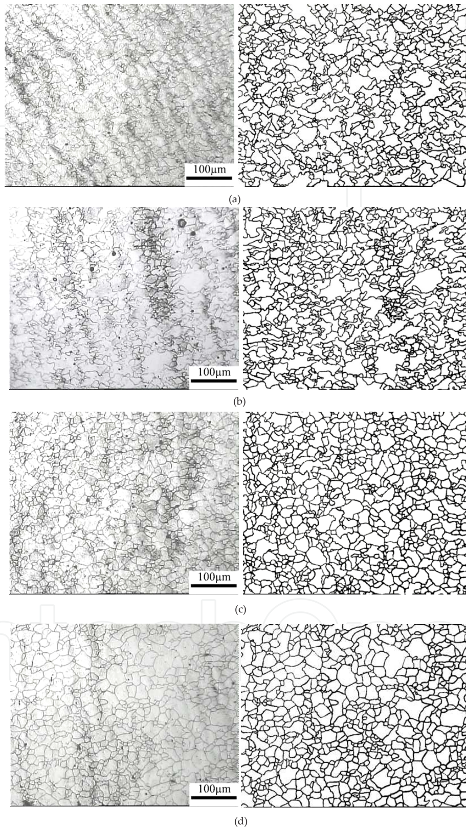
Figure 15. Optical microstructures of 42CrMo high-strength steel at a fixed true strain of 0.9, a fixed temperature of 1198 K and different strain rates: (a) 0.01 \text{ s}^{-1} , (b) 0.1 \text{ s}^{-1} , (c) 1 \text{ s}^{-1} , (d) 10 \text{ s}^{-1} .
