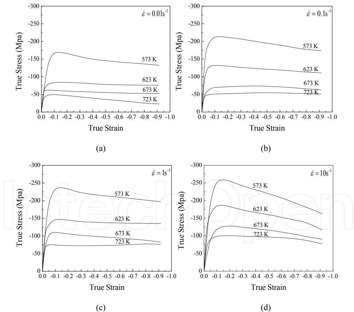
Figure 3. True stress-strain curves of as-extruded 7075 aluminum alloy at different strain rates and temperatures. (a) 0.01 s -1 , 573~723 K, (b) 0.1 s -1 , 573~723 K, (c) 1 s -1 , 573~723 K, (d) 10 s -1 , 573~723 K.
