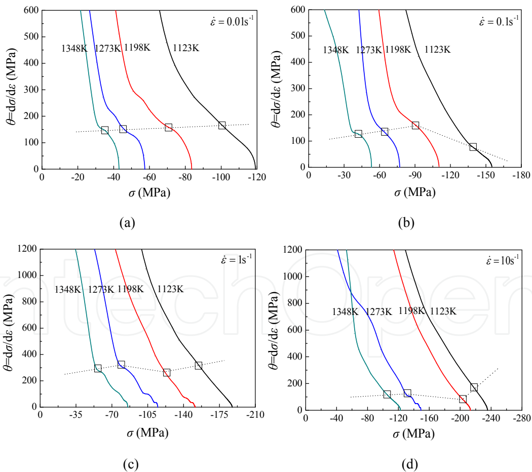
Figure 6. Formula: Eqn012.wmf>versus \frac{d\sigma}{d\varepsilon} plots up to the peak points of the true stress-strain curves under different deformation temperatures with strain rates (a) 0.01 \text{ s}^{-1} , (b) 0.1 \text{ s}^{-1} , (c) 1 \text{ s}^{-1} , (d) 10 \text{ s}^{-1} .
