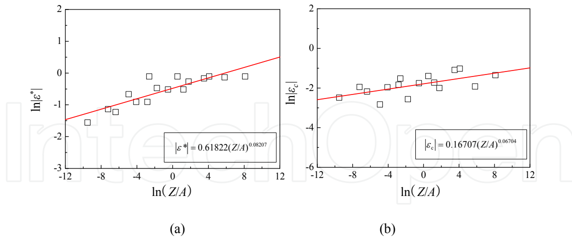
Figure 11. Relationships between the dimensionless parameter, Z/A , and (a) d\sigma / d\epsilon , (b) \sigma .
