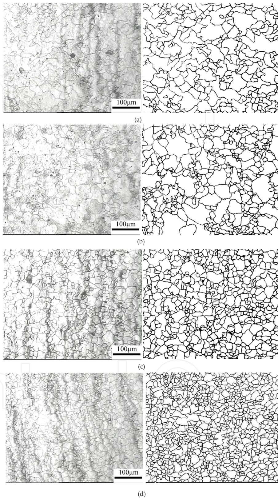
Figure 16. Optical microstructures of 42CrMo high-strength steel at a fixed true strain of 0.9, a fixed temperature of 1273 K and different strain rates: (a) 0.01 \text{ s}^{-1} , (b) 0.1 \text{ s}^{-1} , (c) 1 \text{ s}^{-1} , (d) 10 \text{ s}^{-1} .
