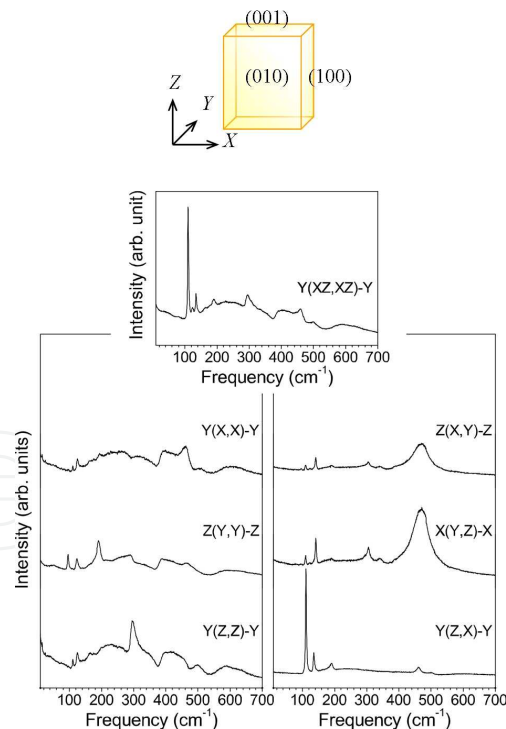
Figure 1. Raman spectra of \text{CdTiO}_3 at room temperature observed with several scattering geometries. See text for configuration notations, for instance Y(X,X)-Y .
