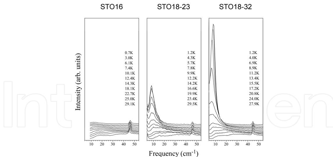
Figure 11. Temperature dependencies of the Raman spectra in STO18- x ( x = 0 [STO16: the pure \text{SrTiO}_3 ], 0.23, and 0.32).
