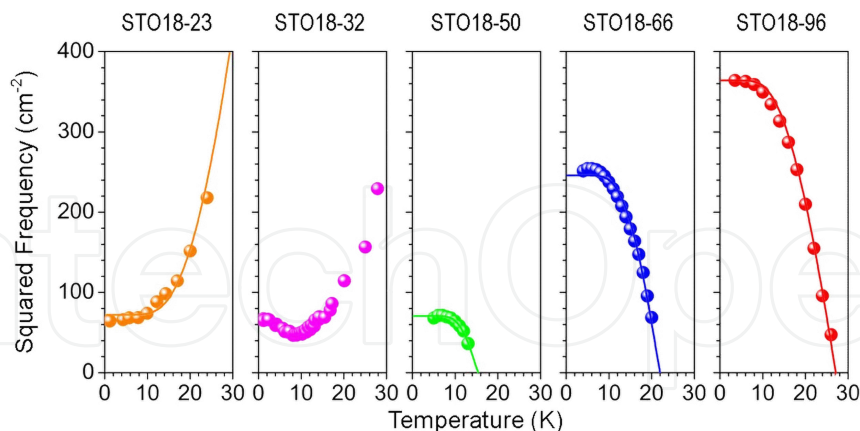
Figure 10. Temperature dependencies of the squared frequencies of the soft mode in STO18- x with various x . Solid lines in the figures denote temperature dependencies calculated by Eq. 3.7 with optimized control parameters (see text).
