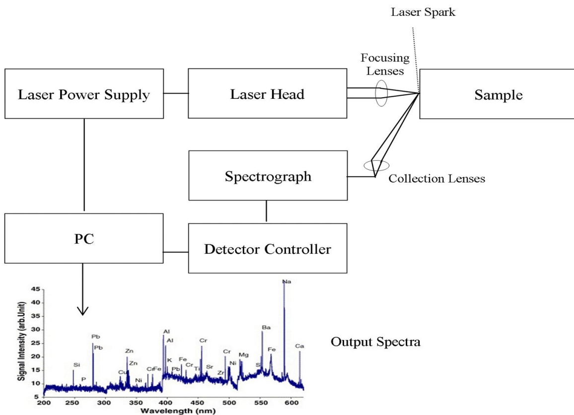
Figure 4. Scheme of an LIBS instrument (Spectra from Reference 48).
