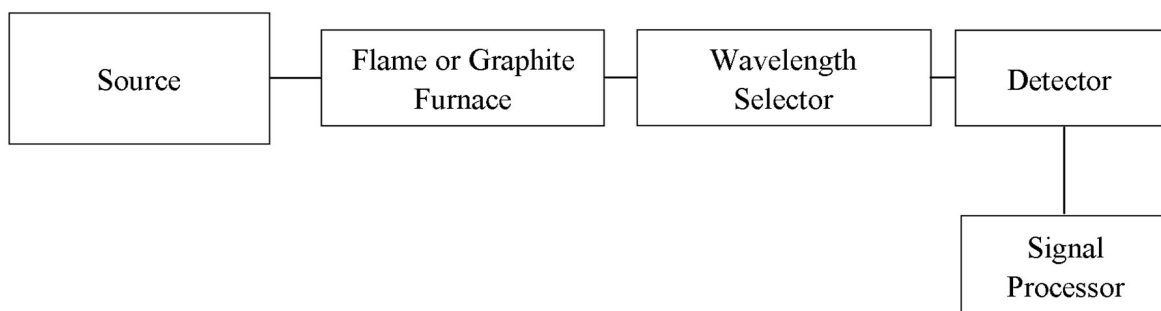
Figure 1. Block Diagram for FAAS and GFAAS.
