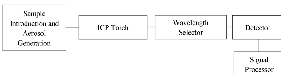
Figure 2. Block Diagram of ICP-OES.
