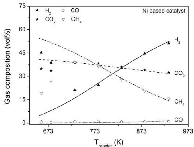
Figure 8. Gas concentration as a function of the temperature for a Ni based catalyst. P = 25.5 - 27.0 MPa, [glycerol] = 10 wt%. The curves represent equilibrium compositions, the symbols are experimental points [29].
