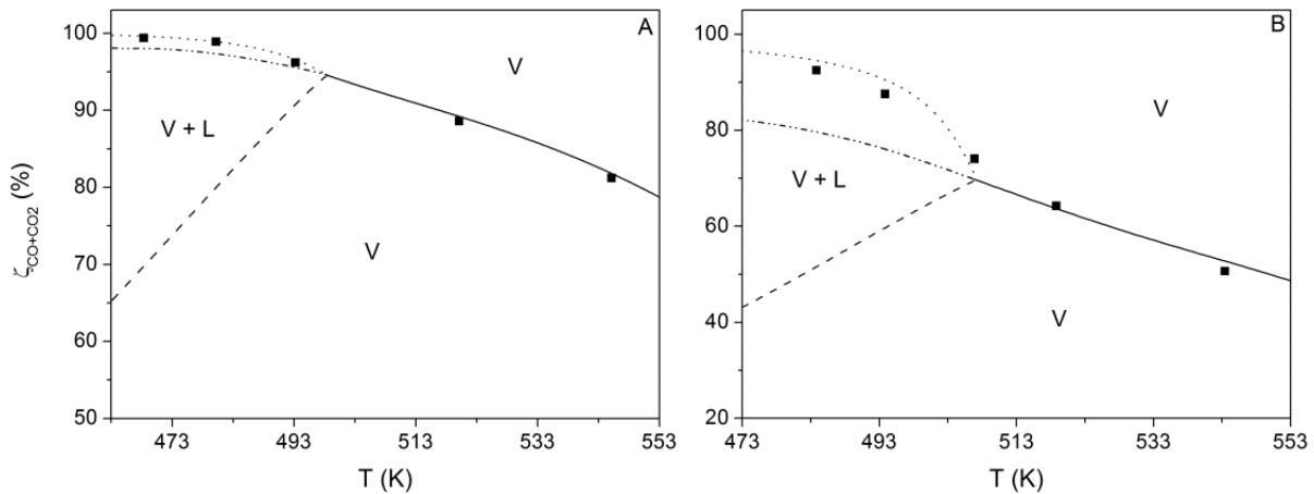
Figure 13. Equilibrium diagrams for methanol synthesis. Gas 1 (A), P = 19.7\text{ MPa} [41]. Gas 2 (B) [45], P = 20.3\text{ MPa} . Symbols: experimental data; curves: model results.
