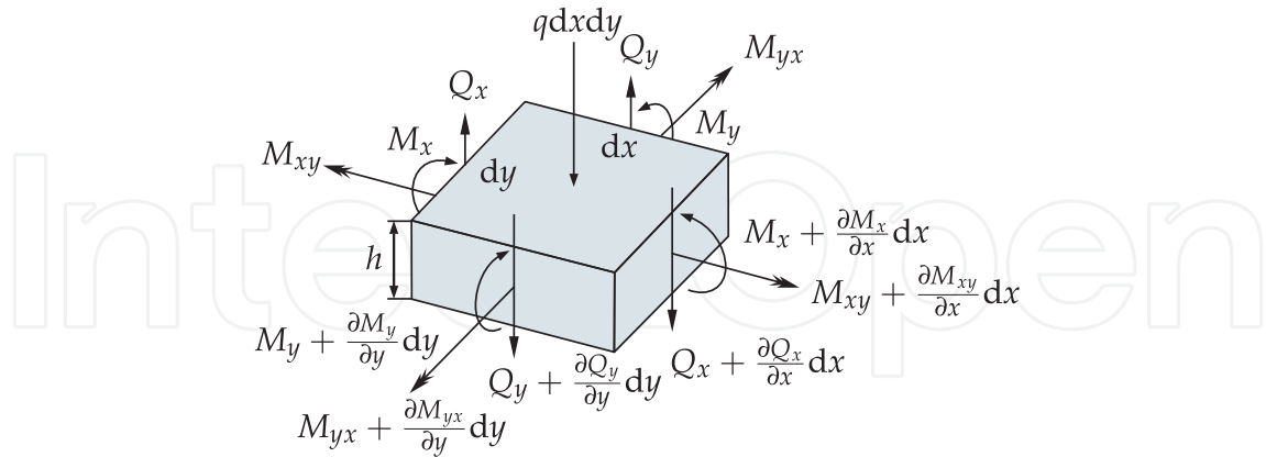
Figure 2. Illustration of shear forces, bending and twisting moments, and external loads affecting a differential plate element h dx dy of the deformable mirror.
