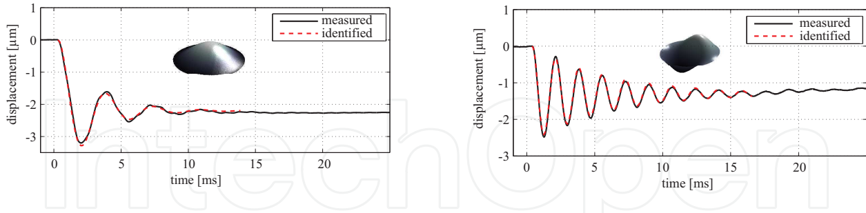
Figure 8. Measured step responses of the first and second eigenfunctions of an Alpa0 DM88 deformable membrane mirror without feedforward control showing a settling time above 5-10 ms
