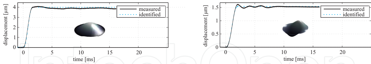
Figure 9. Measured responses of the first and second eigenfunctions of an Alpa0 DM88 deformable membrane mirror with feedforward control showing a settling time of 2 ms
