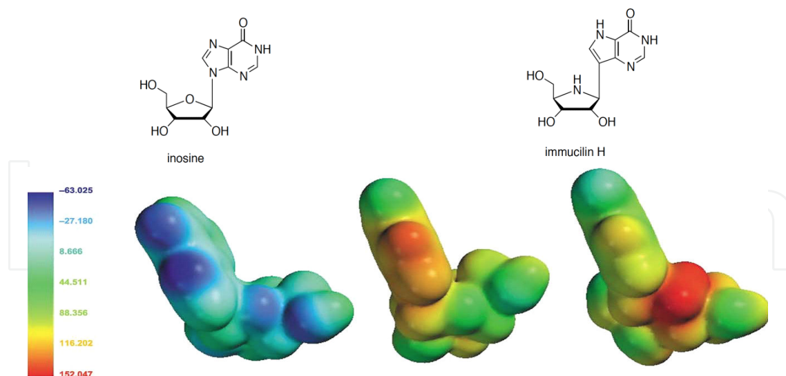
Figure 33. Molecular electrostatic potential surfaces for inosine, the transition state of purine nucleoside phosphorylase and immucilin H.
