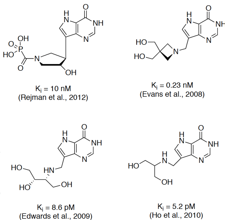
Figure 34. Effective inhibitors of purine nucleotide phosphorylase.
