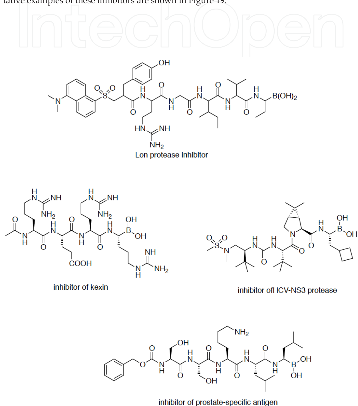
Figure 19. Boronic acid based inhibitors.
