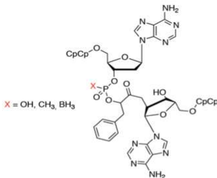
Figure 23. Transition state analog inhibitor of peptidyl transferase.
