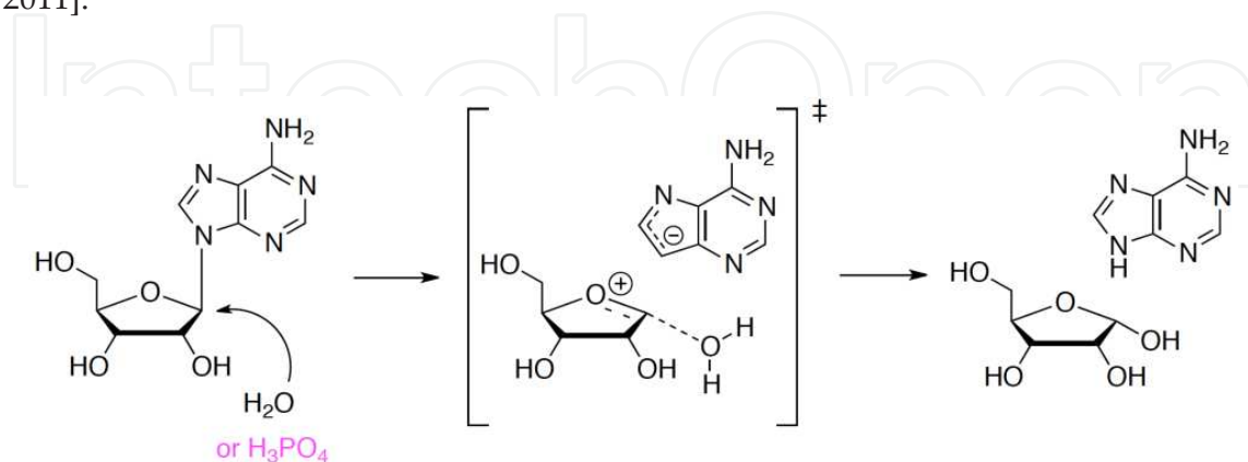
Figure 32. Course of reaction catalyzed by N -ribosyltransferases.
