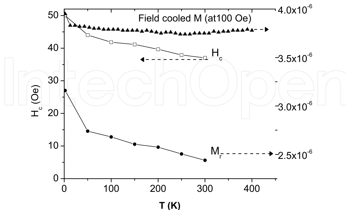
Figure 5. Dependence of remnant magnetization ( M_r ), coercive field ( H_c ) and field cooled magnetization (M-T at 100 Oe) of Zn_{1-x}Mn_xO nanowires on temperature.
