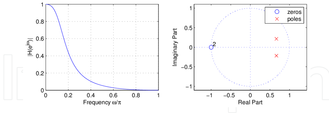
Figure 2. Frequency responses and zero-pole configurations of H(z) .
