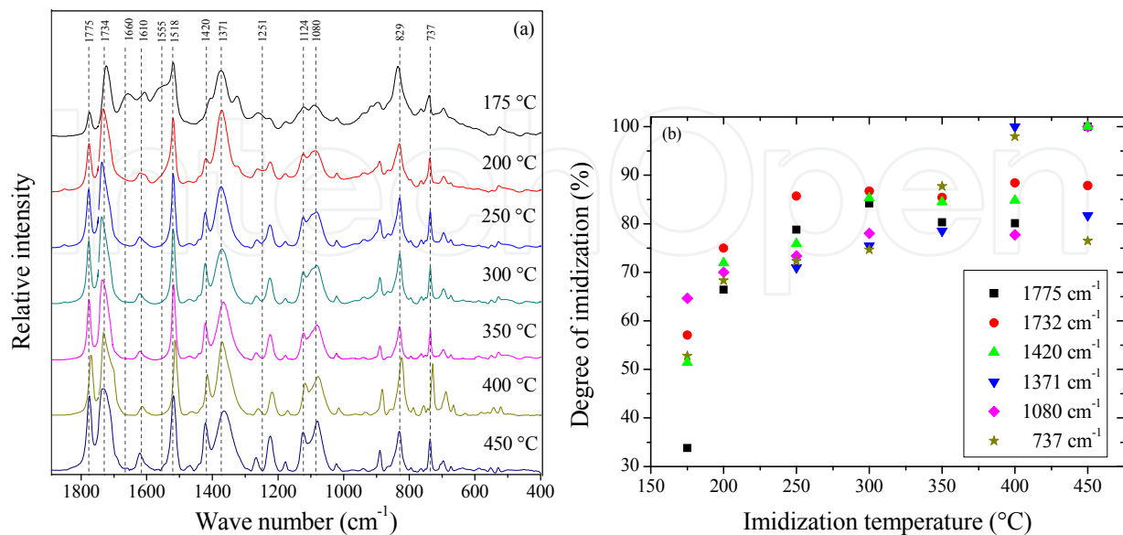
Figure 3. (a) FTIR spectra of BPDA-PDA for different T_{HC} (thickness: 1.5\text{ }\mu\text{m} ). (b) Degree of imidization for the main absorption bands versus the imidization temperature. Taken from [24].
