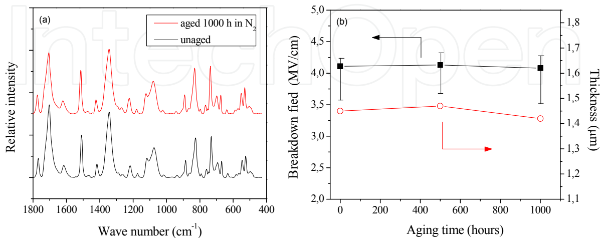
Figure 8. (a) FTIR spectra before and after aging in N 2 at 300 °C and (b) breakdown field and thickness during aging for 1.5 μm-thick BPDA-PDA films. The breakdown field is measured at 300 °C.
