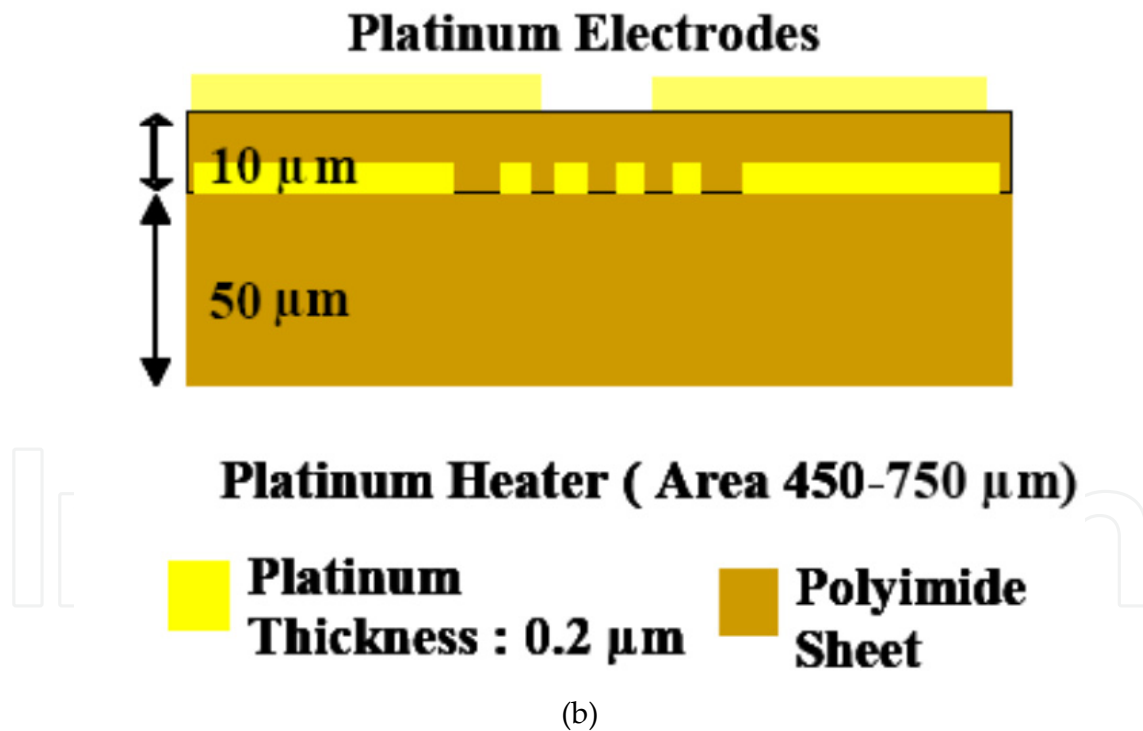
Figure 3. (a) Design of the gas sensing structure realised using the both sides of a polyimide sheet. (b) Design of the gas sensing structure realised only on the top side of the polyimide sheet[37].
