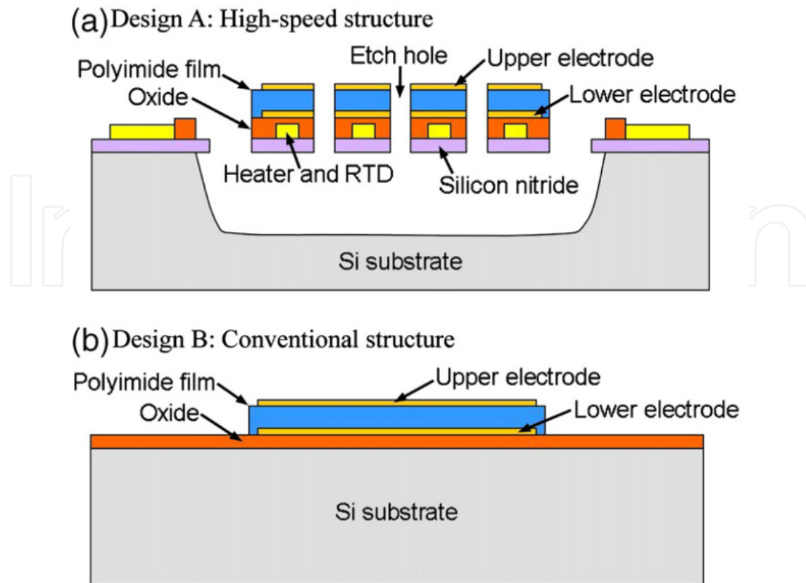
Figure 6. Schematic cross-sectional views of two capacitive humidity sensors (a) Design A: High-speed structure (b) Design B: Conventional structure[42].
