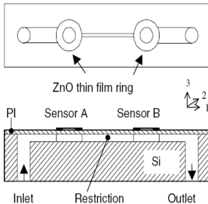
Figure 10. Schematic view of the device[48].
