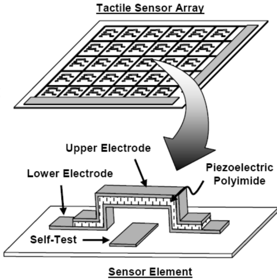
Figure 7. Tactile sensor array and an individual polyimide sensor element.[44]
