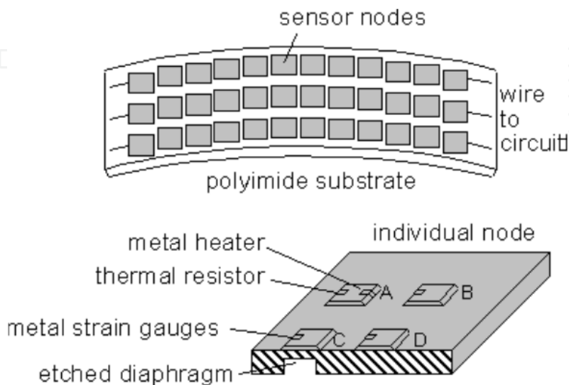
Figure 8. Schematic diagram of the polyimide multimodal tactile sensor[45].
