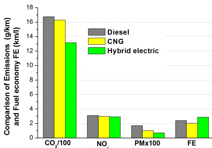
Figure 8. Comparison between the different bus technologies.
