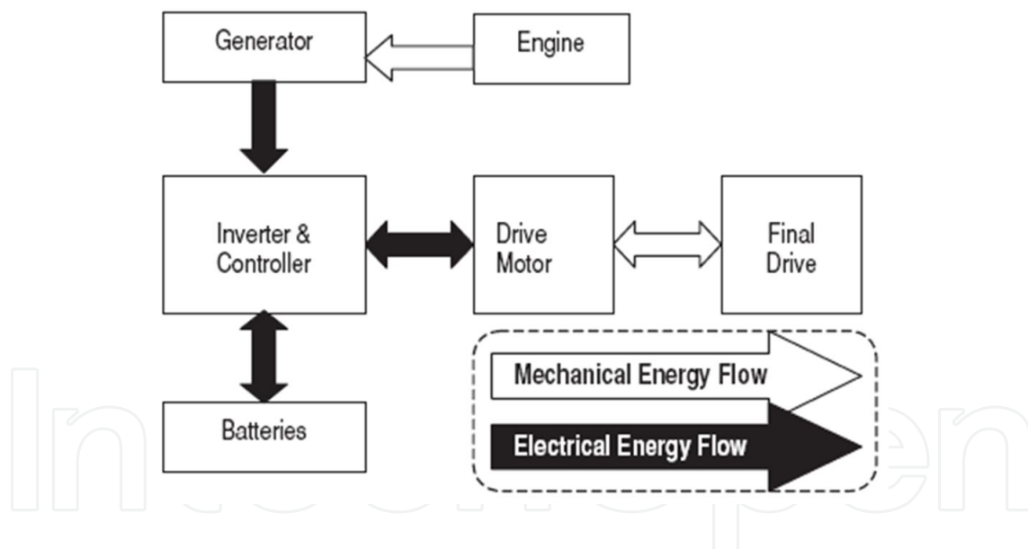
Figure 2. Series hybrid electric drive system.
