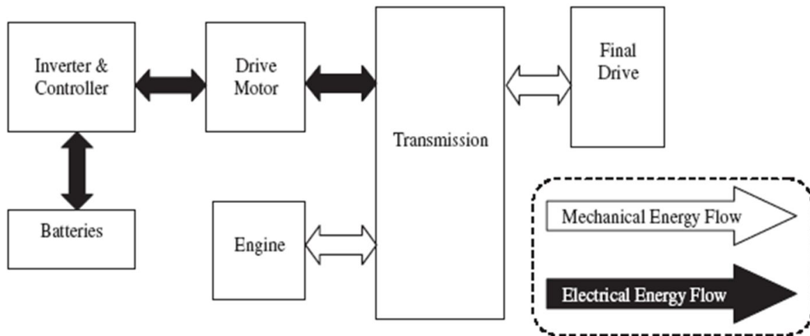
Figure 3. Parallel hybrid electric drive system.
