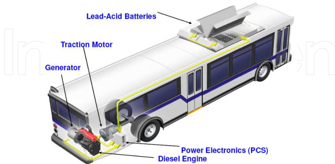
Figure 6. Series hybrid propulsion system.
