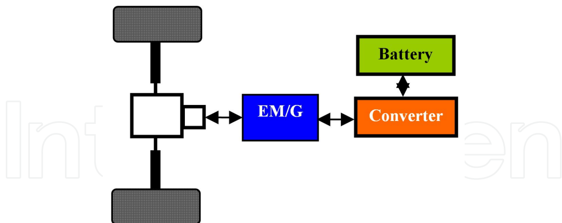
Figure 4. Battery electric drive system.
