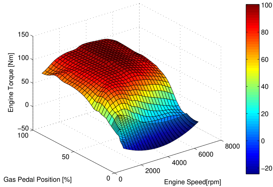
Figure 17. Engine torque map.
