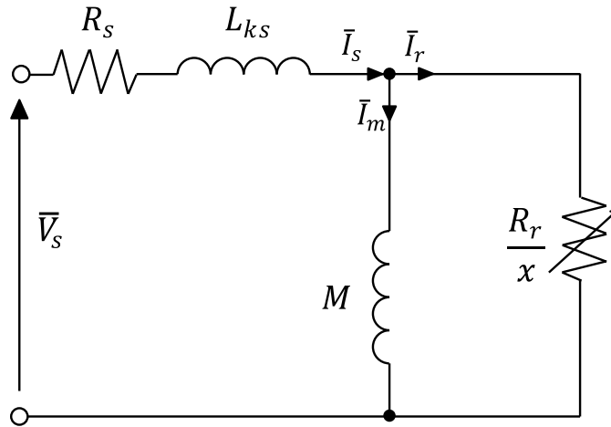
Figure 14. Induction motor steady-state equivalent circuit.
