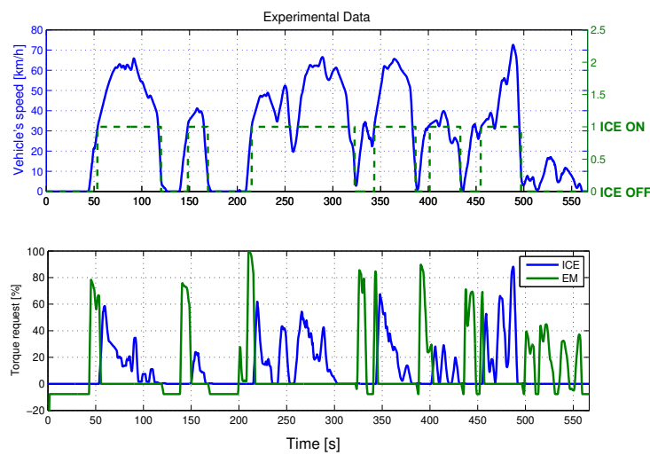
Figure 28. Drive cycle with superimposed the ICE status
