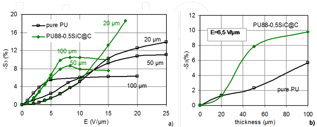
Figure 19. Evolution of the strain amplitude versus the electric field amplitude for various thicknesses of pure PU88 and PU88-0.5SiC@C films at 0.1 Hz. (b) The evolution of the strain amplitude versus the thickness of pure PU88 and PU88-0.5SiC@C films at E = 6.5 \text{ V}/\mu\text{m} [11]
