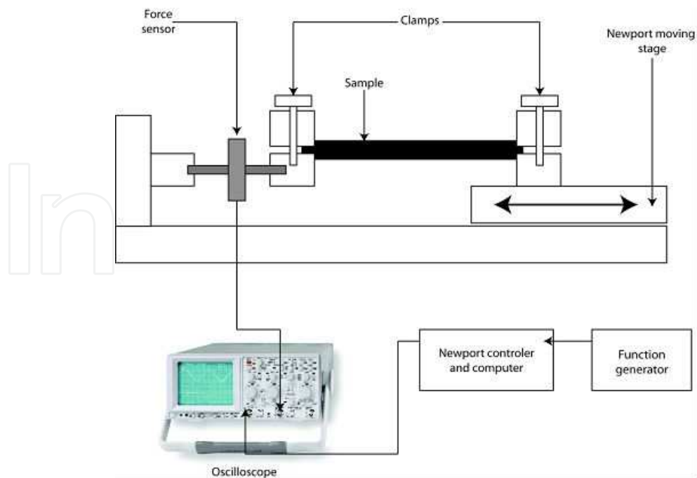
Figure 16. Experimental set-up for measuring the mechanical properties of the nanocomposite films
