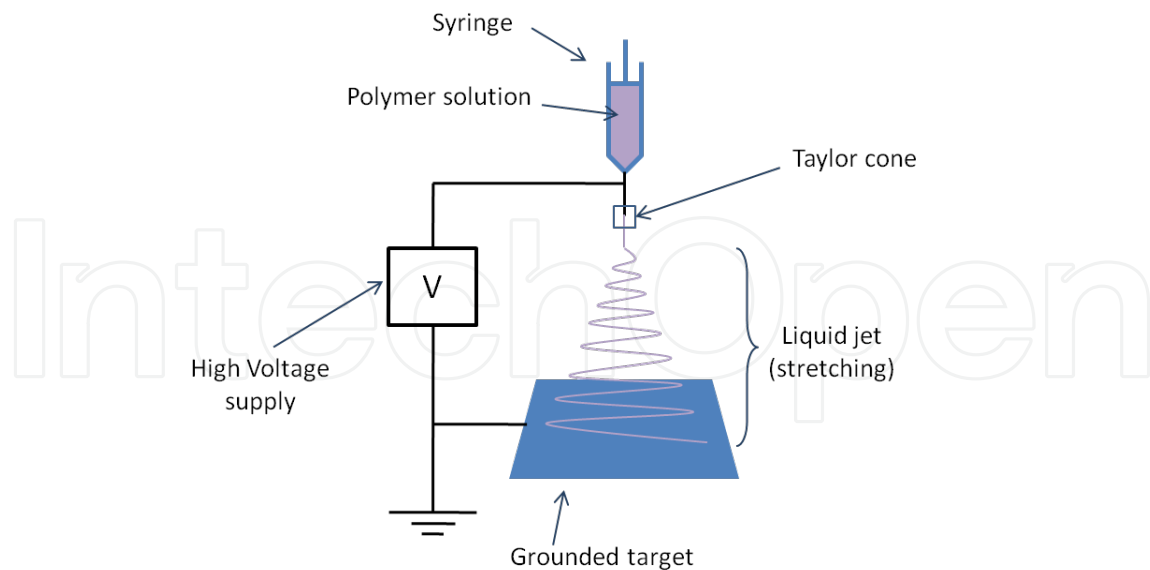
Figure 5. Schema of a typical electrospinning setup
