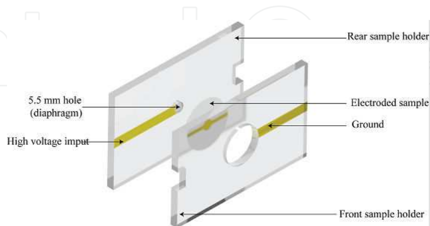
Figure 20. Diaphragm device used for the measurement of the deflection strain under electrical field at high frequency [35]
