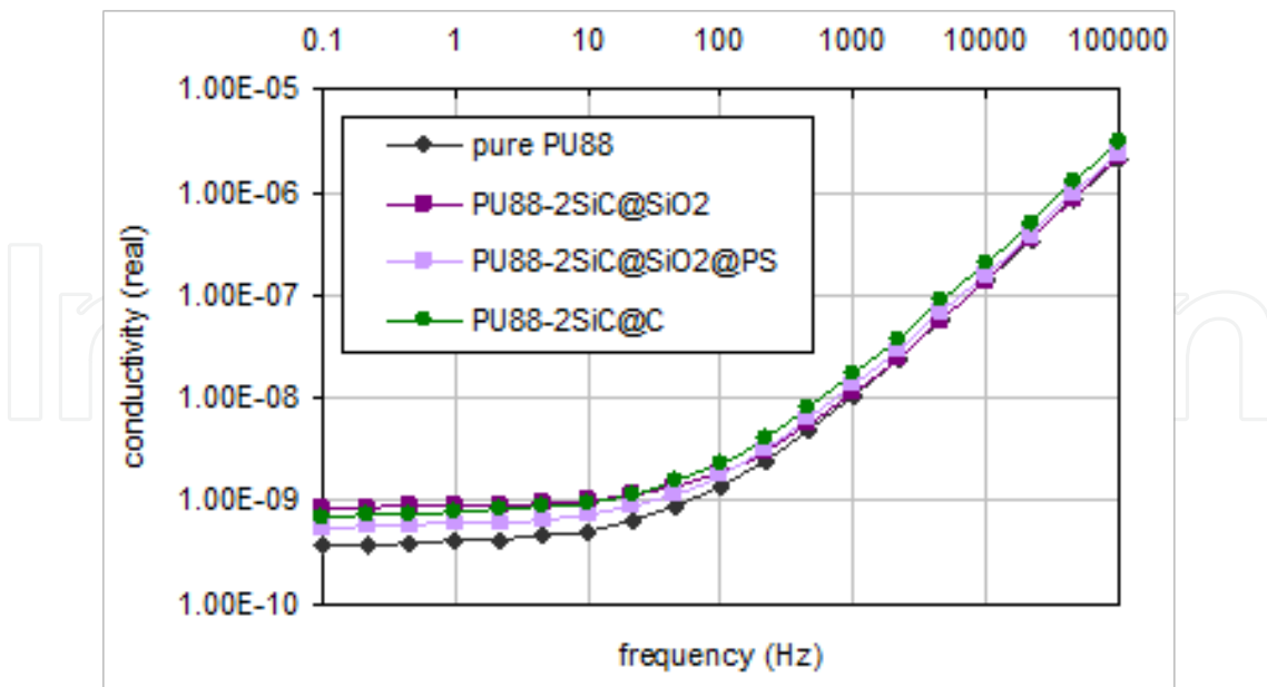
Figure 13. The electrical conductivity versus frequency for pure PU and PU88-2SiC composites
