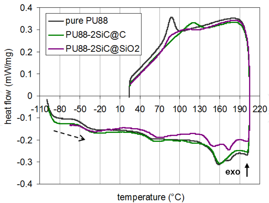
Figure 12. DSC thermograms on heating and cooling of pure PU88, PU88-2SiC@C and PU88-2SiC@SiO 2 nanocomposites films
