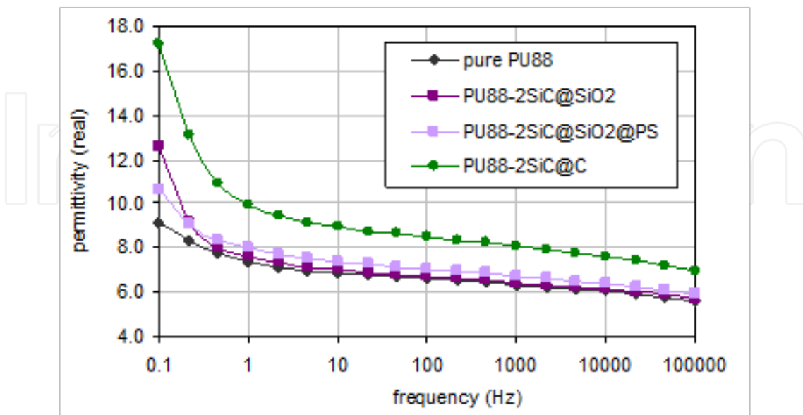
Figure 14. The relative permittivity versus frequency for pure PU and PU88-2SiC composites.
