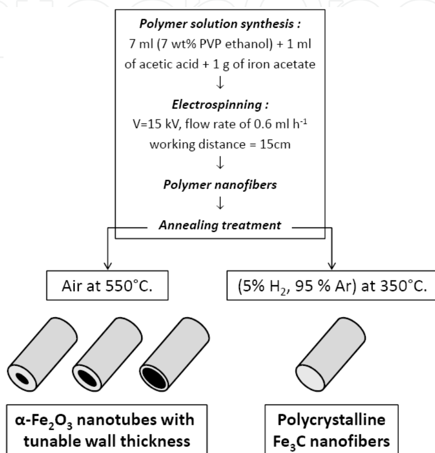
Figure 6. Experimental process with the different nanostructures obtained [25]
