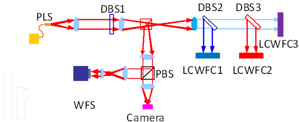
Figure 22. Optical set-up for a broadband correction - PLS represents a point light source, PBS is a polarized beam splitter, DBS means dichroic beam splitter, DBS1 is a band-pass filter, and DBS2 and DBS3 are long-pass filters.
