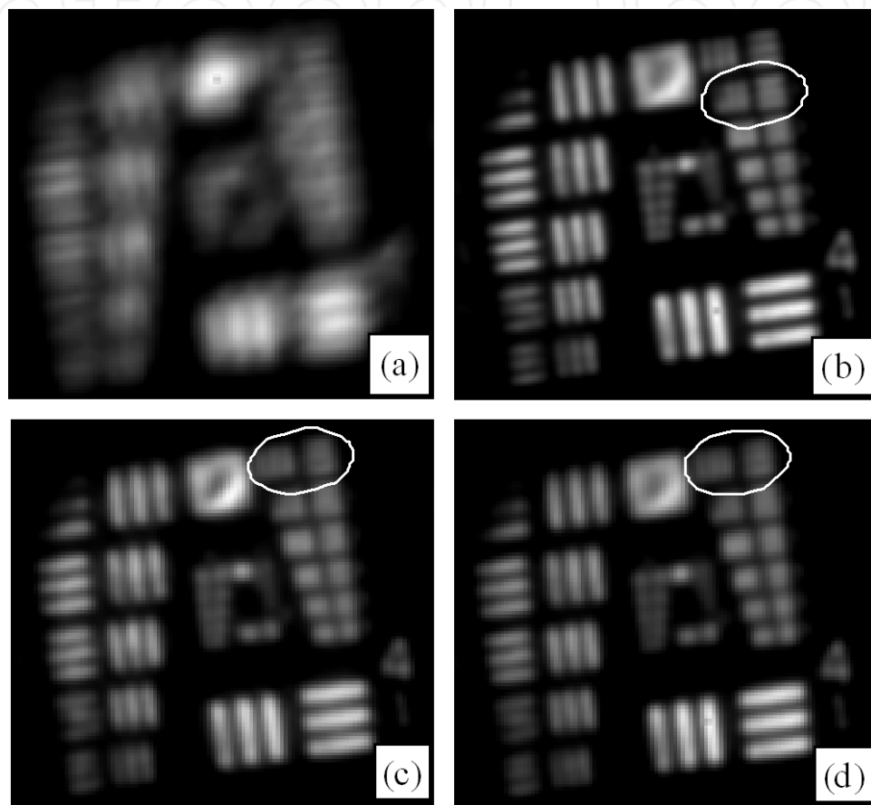
Figure 23. Images of the resolution target for different wavebands: (a) no correction; (b) 520–590 nm; (c) 590–690 nm; (d) 520–690 nm - the circular area represent the resolving limitation.
