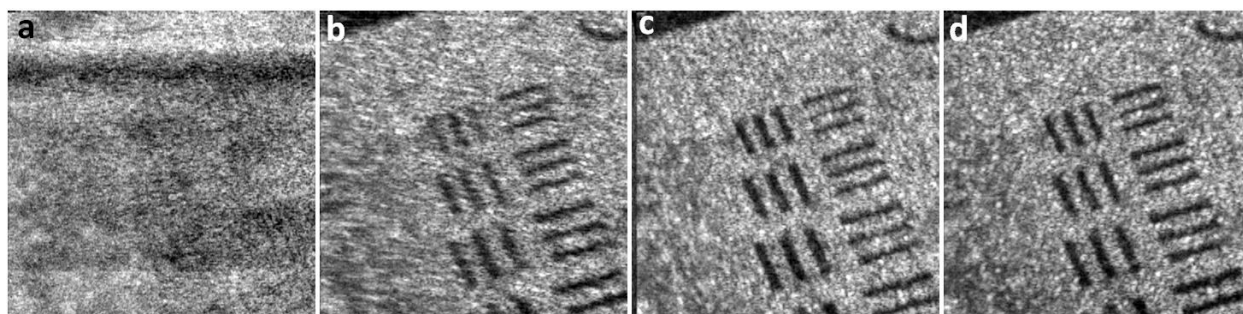
Figure 14. En-face projection views of the AO-OCT images of the test target for the best corrected values of the Zernike coefficients; (a) before correction, (b) after defocus correction, (c) after defocus and Ast 0^\circ correction, (d) after defocus, Ast 0^\circ and Ast 45^\circ correction.
