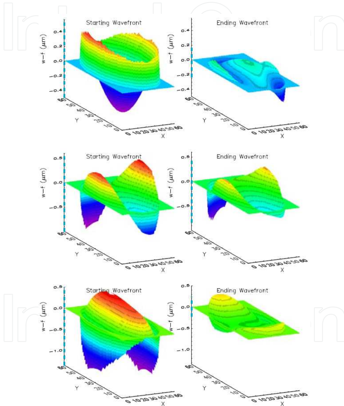
Figure 11. Wavefront plots (obtained with the wavefront analysis, WFA) before and after the correction applied by the deformable mirror for three considered cases. Top: the main aberration is defocus; Middle: the main aberrations are astigmatism and coma; Bottom: the main aberrations are defocus and astigmatism. The blue dashed lines overplotted to the Z axis represent the total wavefront excursion.
